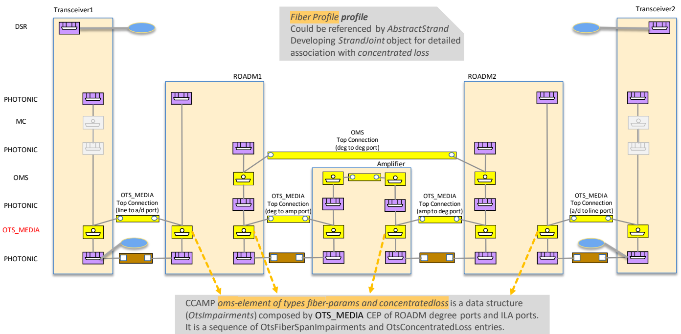
Figure 6-85 OTS Impairments
