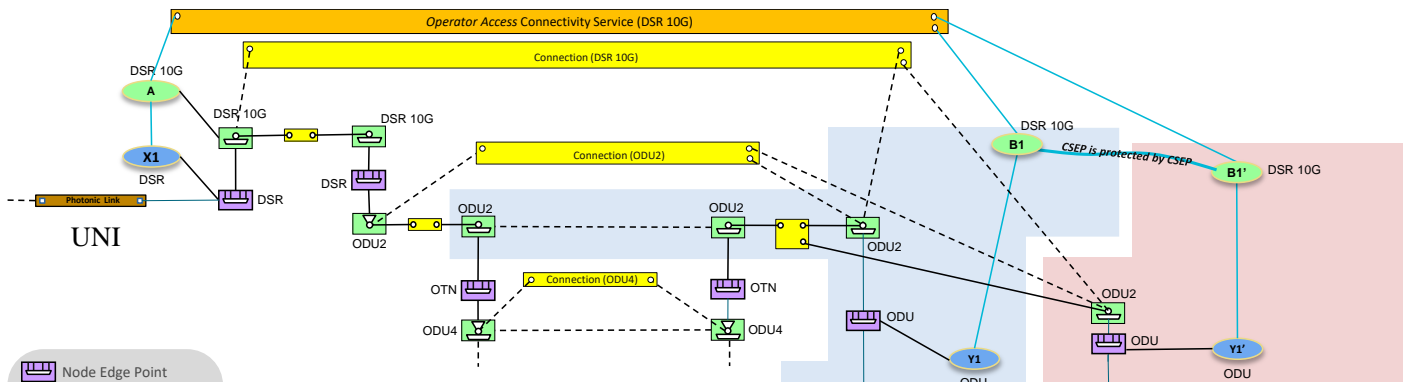
Figure 6-77 TAPI context after asymmetric connectivity-service with 1+1 Protection with Diverse Service Provisioning (eSNCP) provisioning between UNI DSR and E-NNI OTUk interfaces.
