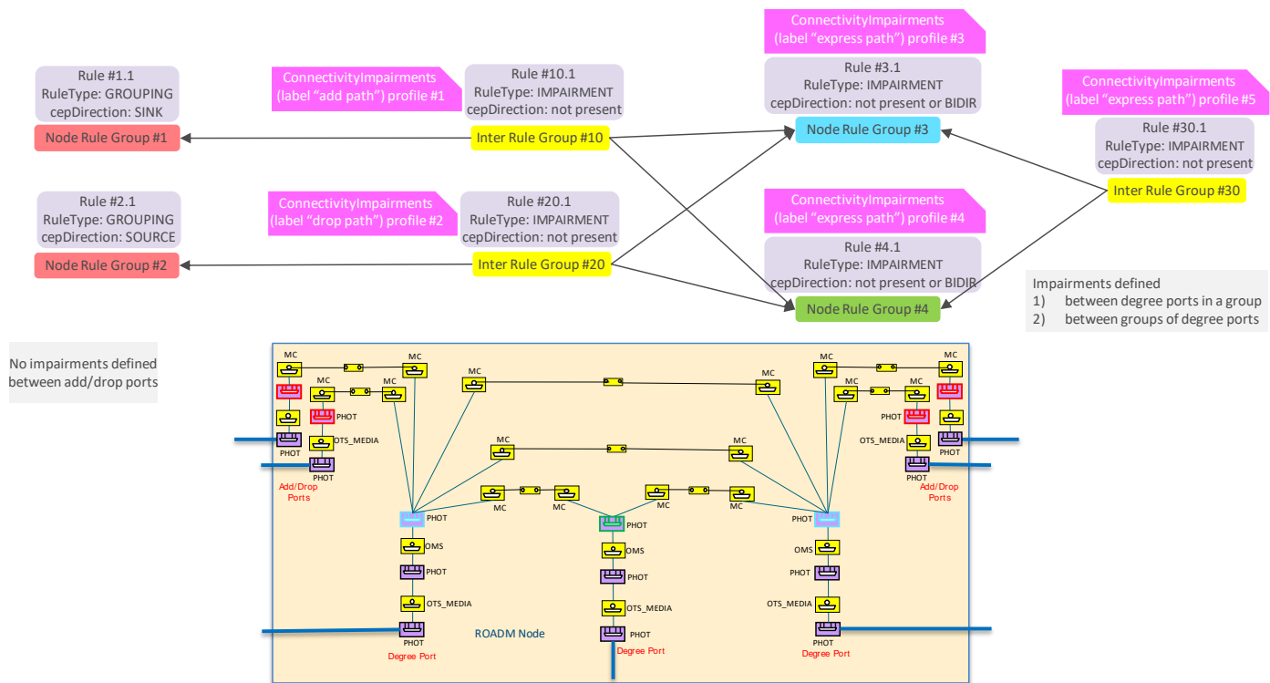
Figure 6-92 Conn. Impairments specified per add , drop and express conns, not homogeneous between express
