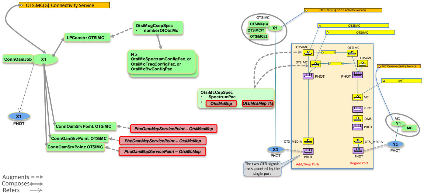
Figure 6-51 OTSiMC(G) CS on MC CS at Degree side
