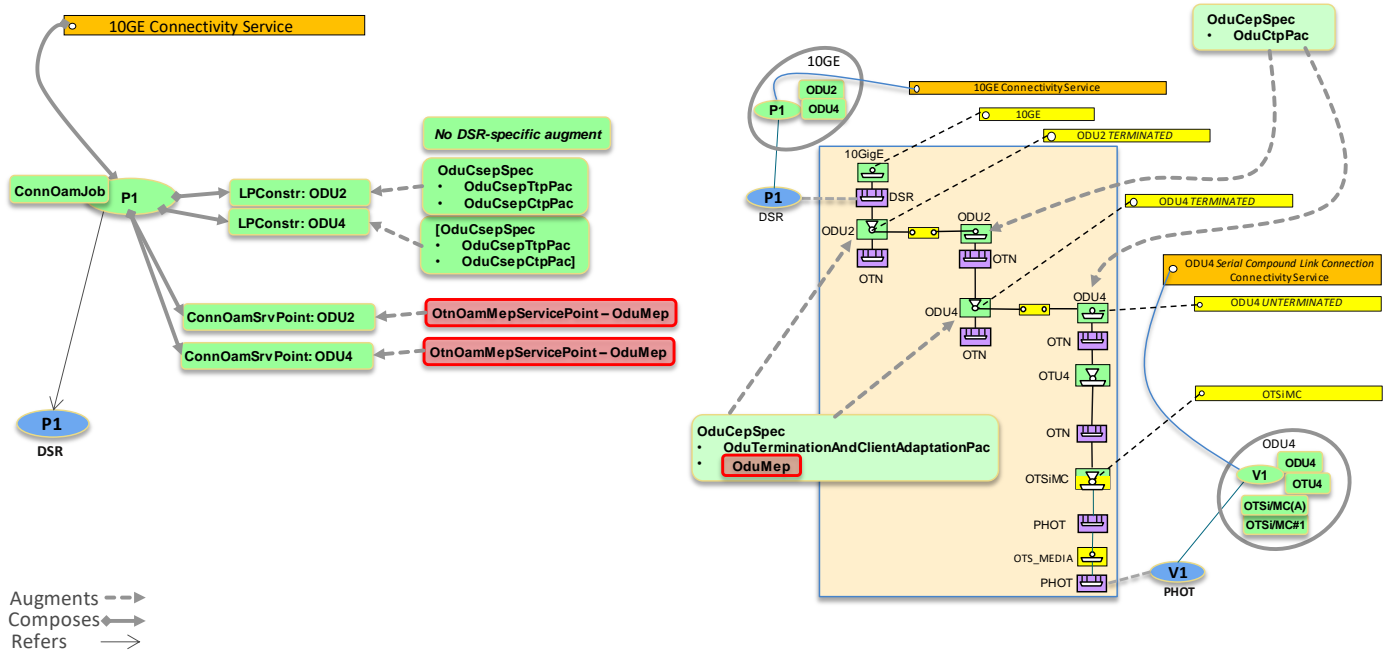
Figure 6-10 DSR/ODUj CS on ODUk SCLC CS, ODUk Terminated Connection automatically created or reused
