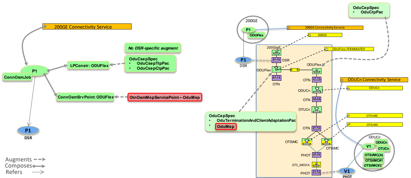
Figure 6-34 DSR/ODUFlex Connectivity Service on ODUcN CS
