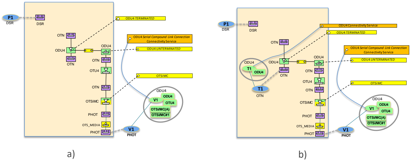
Figure 6-55 a) Server ODU SCLC CS and HO ODU connection, b) Server ODU SCLC CS and HO ODU CS
