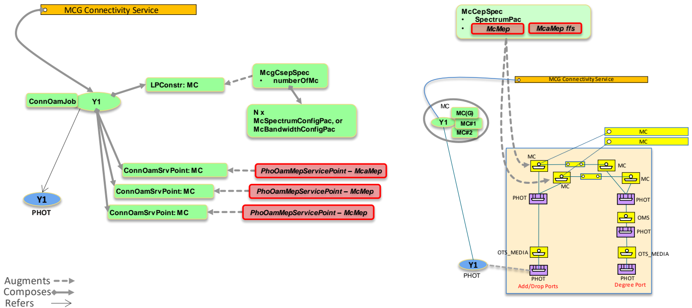
Figure 6-43 MCG Connectivity Service at Add/Drop side
