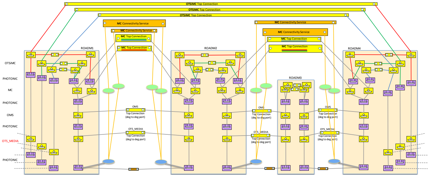
Figure 5-33 Scenario 2 : Integrated Management, sequence of MC top-connections
