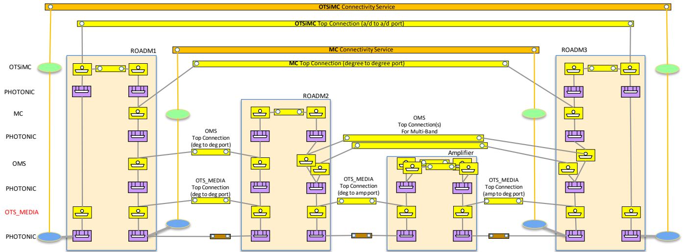
Figure 5-15 Scenario 1 : Optical Line System Controller, multi-band, and SIPs at degree ports
