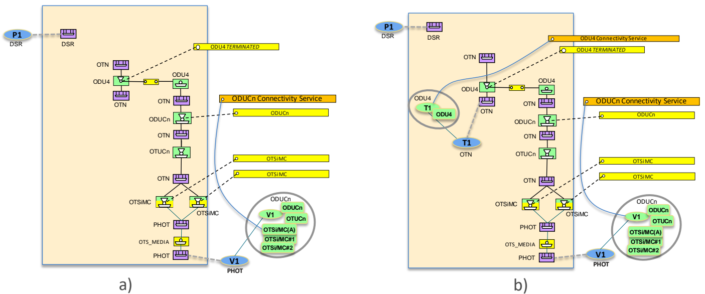
Figure 6-57 a) No server connections, b) Server ODUcN Connectivity Service
