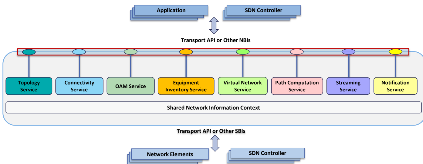
Figure 3-1 Transport API Functional Architecture
