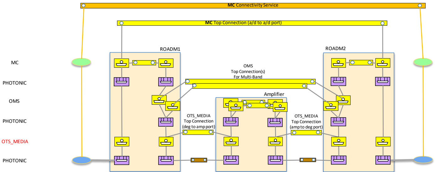
Figure 5-14 Scenario 1 : Optical Line System Controller, multi-band (note: not all MC NEPs are represented)
