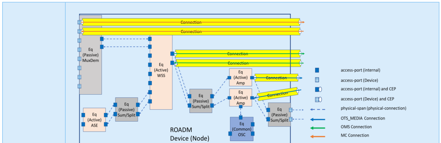
Figure 6-4: TOP Connection and Equipment within a ROADM Device
