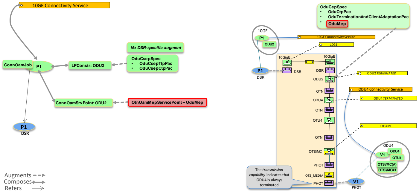
Figure 6-41 DSR CS on ODUj on ODUk CS (DSR flexibility)
