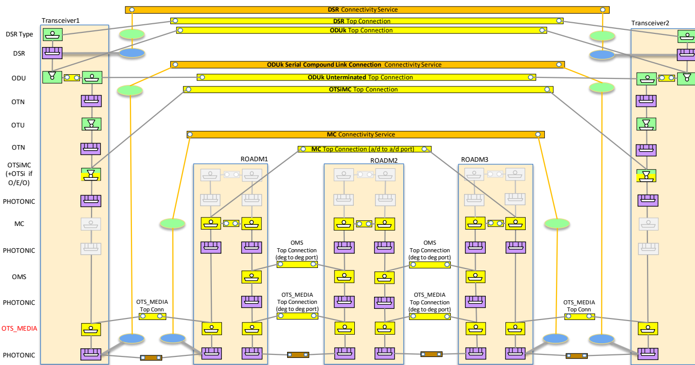
Figure 5-23 Scenario 2 : Integrated Management, MC and OTSiMC+ODU and DSR CSs, OTSiMC CEPs
