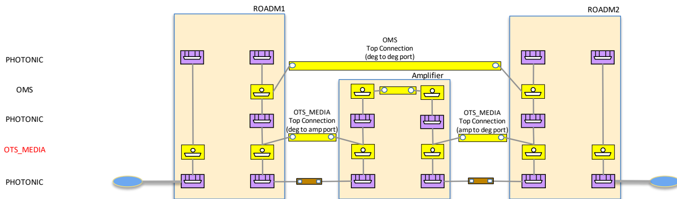
Figure 5-7 Scenario 1 : Optical Line System Controller, time zero, In Line Amplifier
