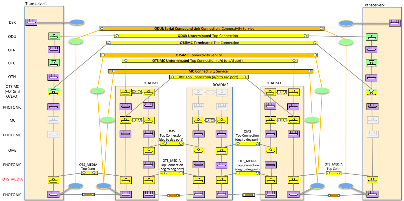
Figure 5-24 Scenario 2 : Integrated Mng, MC CS, unterminated OTSiMC CS, terminated OTSiMC +ODU CSs
