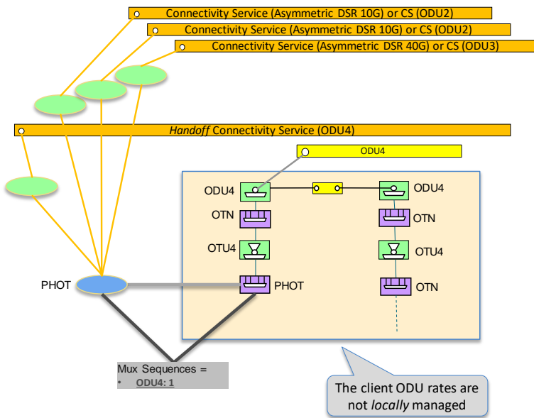
Figure 5-53 OTN ENNI, not locally mapped & multiplexed client protocols, with OTU CEP
