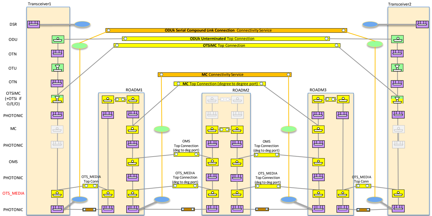
Figure 5-28 Scenario 2 : Integrated Management, MC and OTSiMC+ODU CSs
