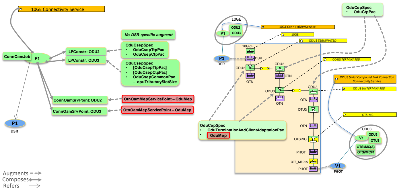
Figure 6-11 DSR/ODU2 CS on ODU3 SCLC CS, ODU3 Terminated Connection automatically created or reused
