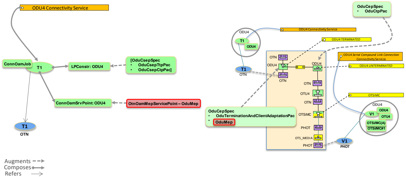
Figure 6-14 Infrastructure or Handoff ODUk Connectivity Service on ODUk SCLC CS
