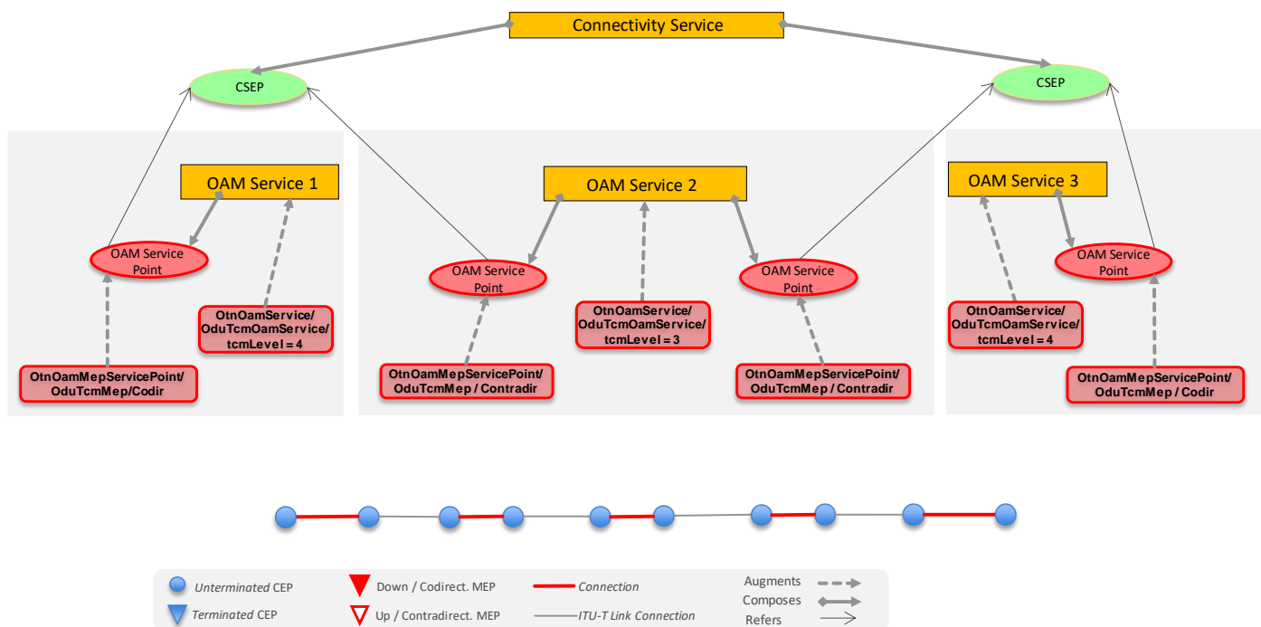
Figure 6-99 OAM provisioning, Client Controller creates the OAM Service and its End Points, OTN NNI to NNI
