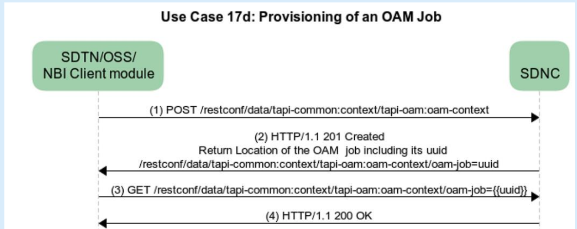
Figure 6-109 UC-17d: Creation and subsequent retrieval of an OAM Job
