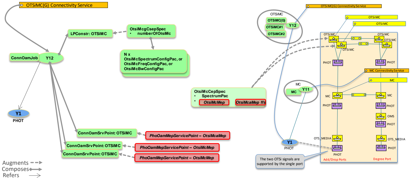
Figure 6-46 OTSiMCG CS on MC CS at Add/Drop side
