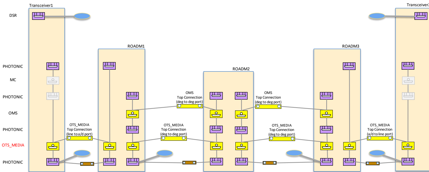
Figure 5-26 Scenario 2 : Integrated Management, time zero, SIPs at ROADM degree ports
