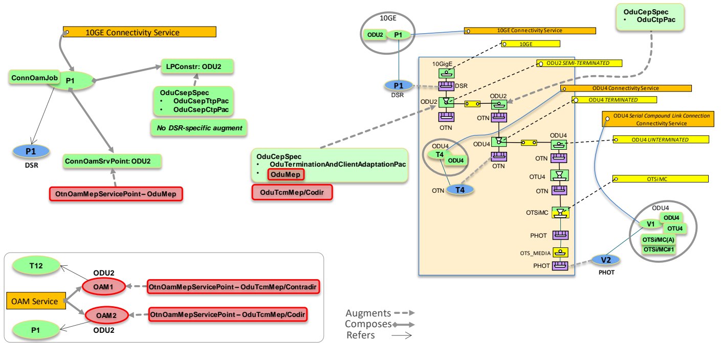
Figure 6-24 Asymmetric scenario 1: DSR/ODUj CS (DSR UNI)
