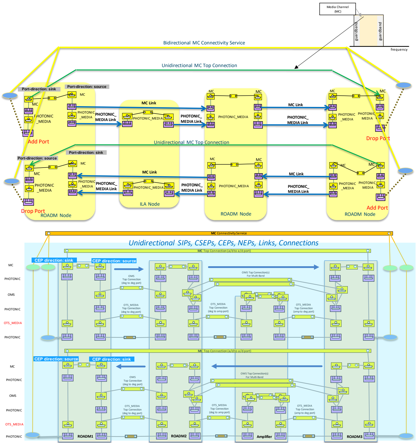
Figure 6-62 Full Unidirectional - UNI and OMS unidirectional scenario.
