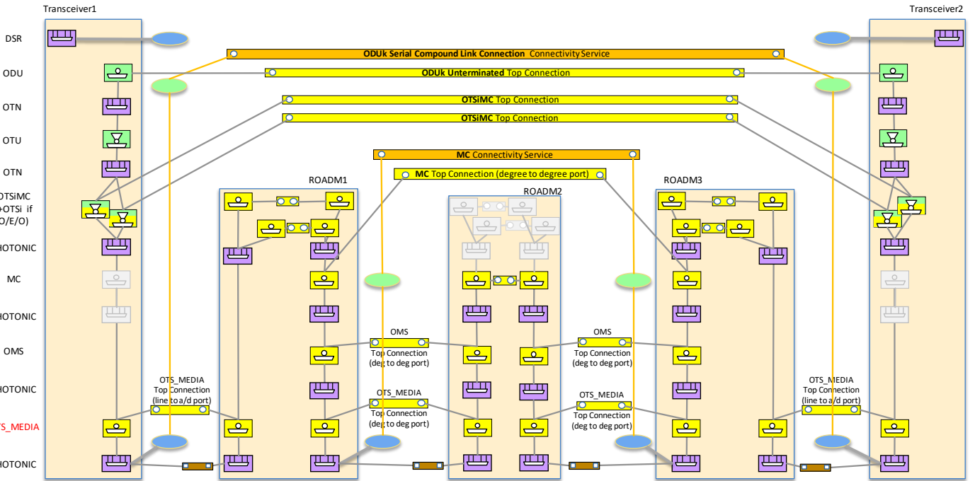
Figure 5-31 Scenario 2 : Integrated Management, MC and OTSiMC+ODU CSs, more OTSiMCs on MC, single line port
