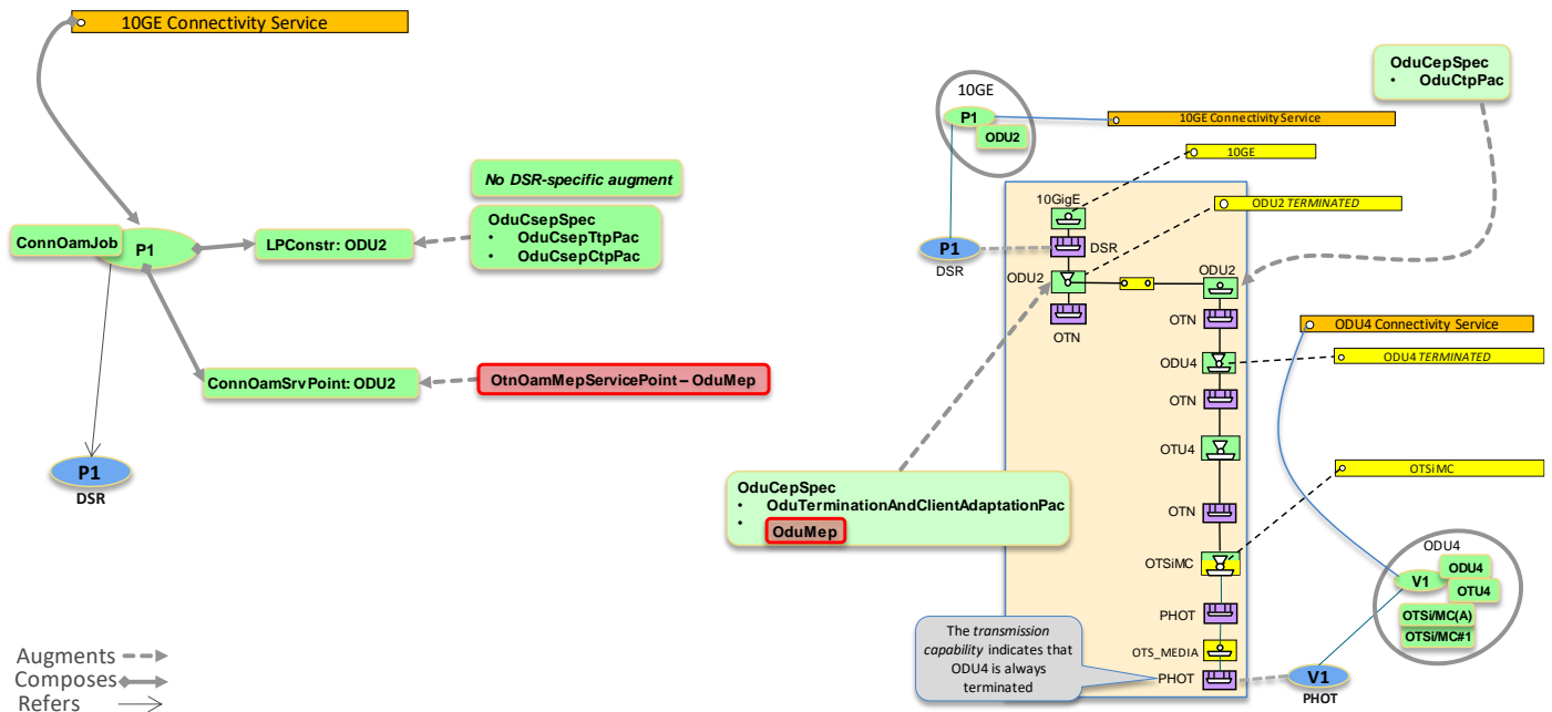
Figure 6-40 DSR/ODUj CS on ODUk CS
