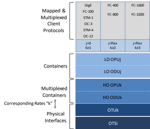
MEF 64 Figure 6 – OTUk Structure for Mapped & Multiplexed Client Protocols
