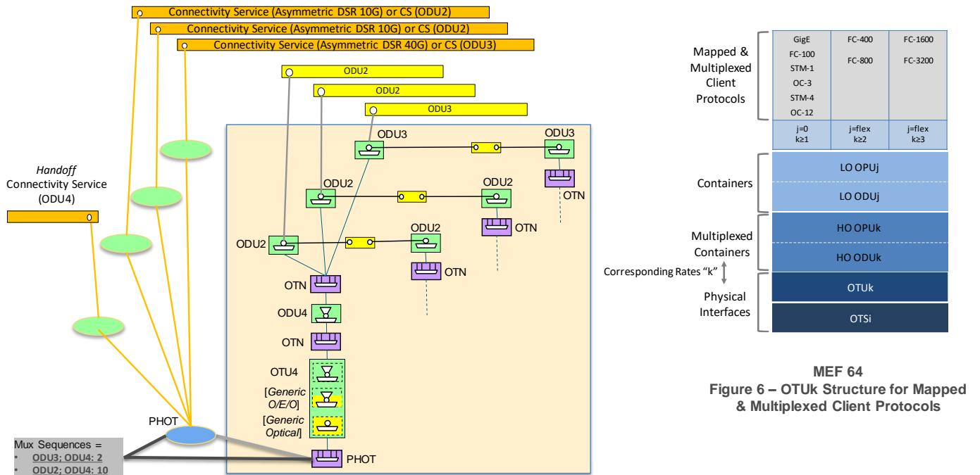
Figure 5-51 OTN ENNI, mapped & multiplexed client protocols, with additional embedded functions of OTU CEP
