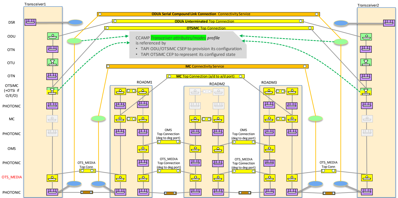
Figure 6-83 Transceiver Profile, configuration and state
