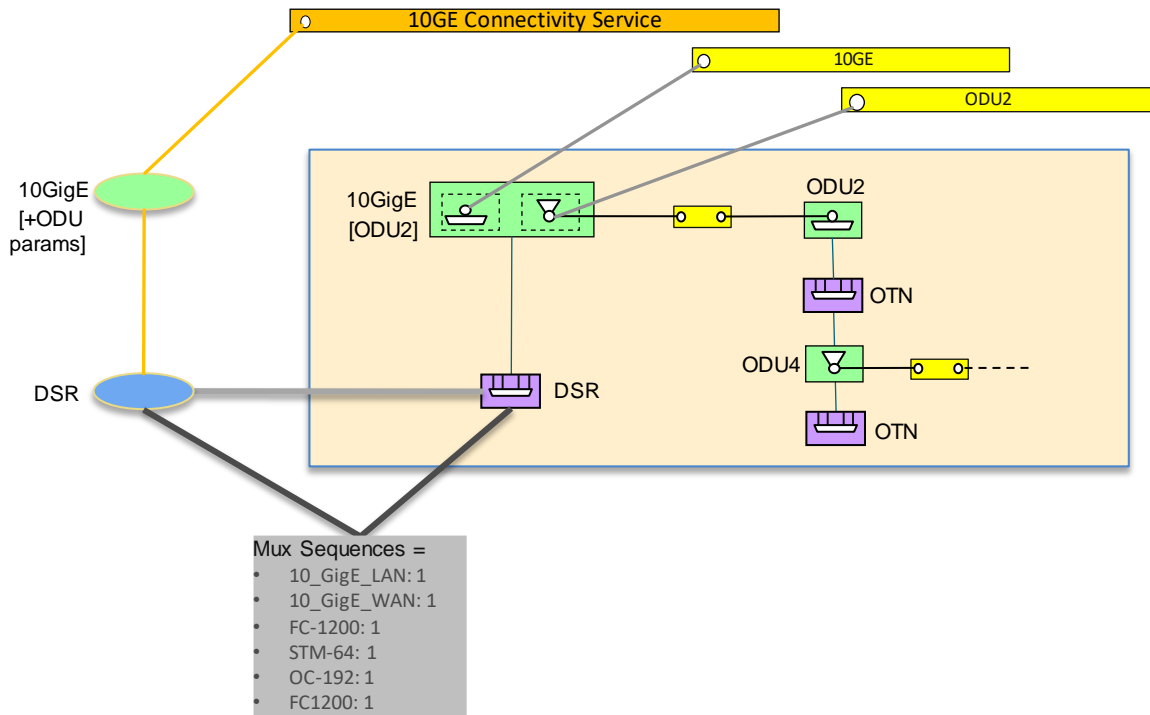
Figure 5-39 Option: Simplified DSR UNI
