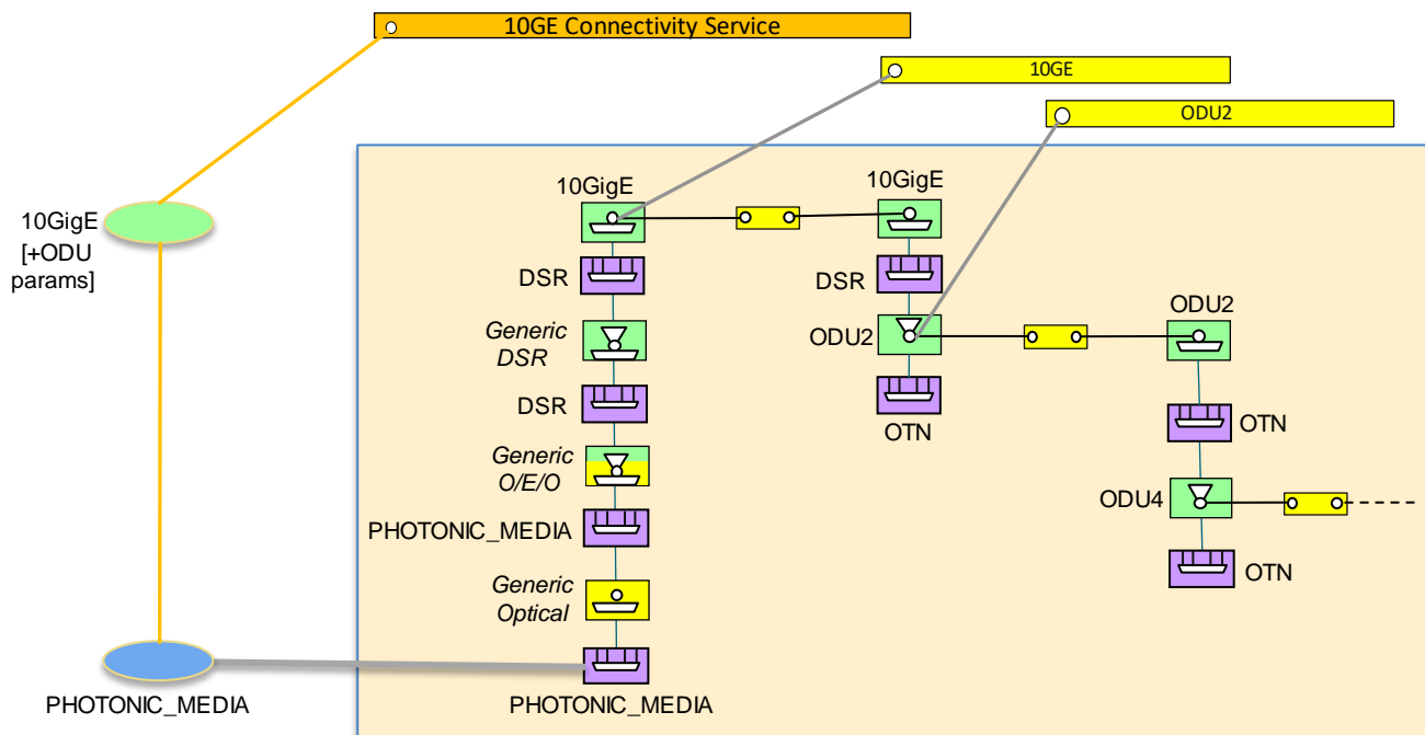
Figure 5-43 DSR UNI, explicit model of functions (optical)
