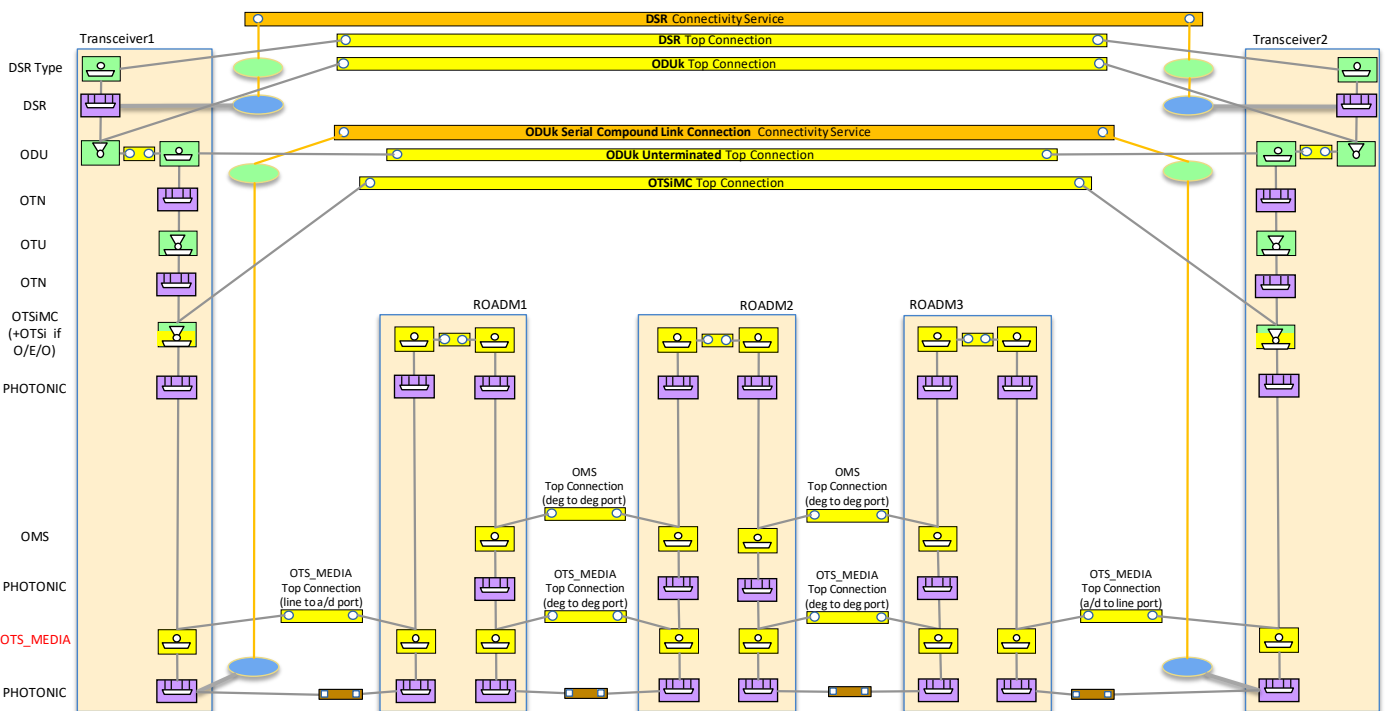
Figure 5-32 Scenario 2 : Integrated Management, MC and OTSiMC+ODU CSs, MC not represented
