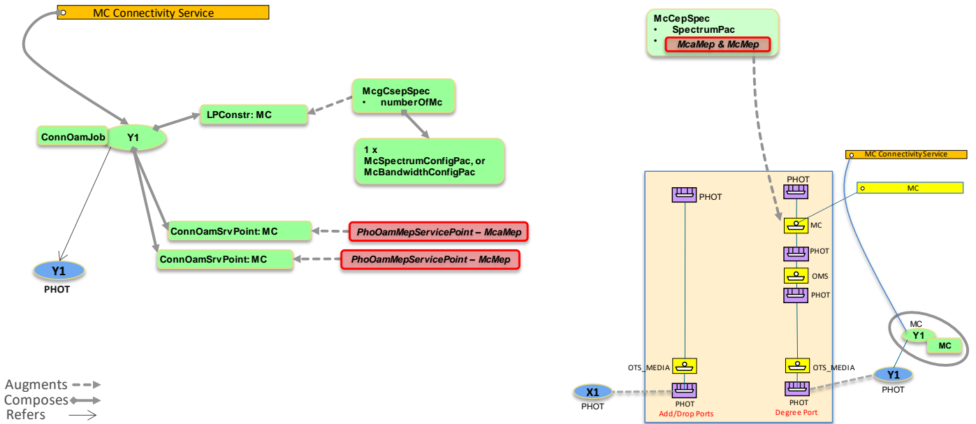
Figure 6-47 MC Connectivity Service at Degree side
