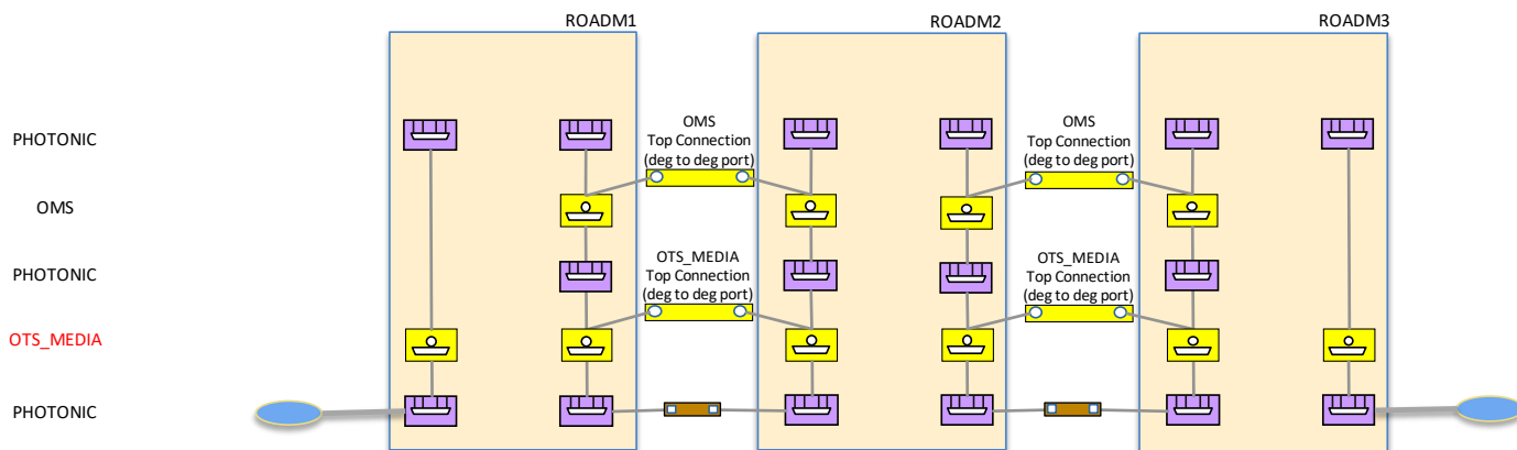
Figure 5-6 Scenario 1 : Optical Line System Controller, time zero
