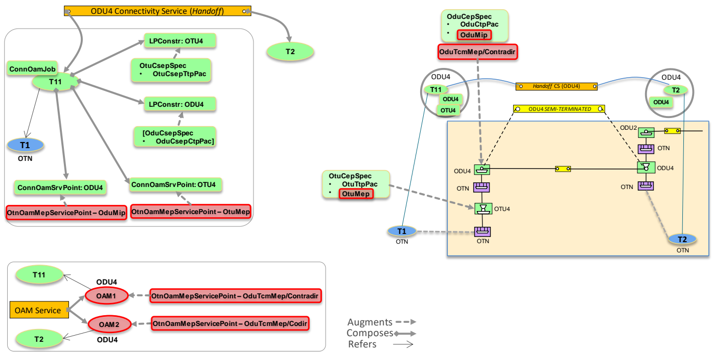
Figure 6-25 Asymmetric scenario 2: ODUk Handoff CS (OTN ENNI) - Part 1
