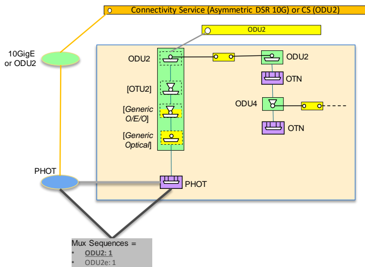
Figure 5-47 OTN ENNI, directly mapped client protocols, with additional embedded functions, 10GE/ODU2
