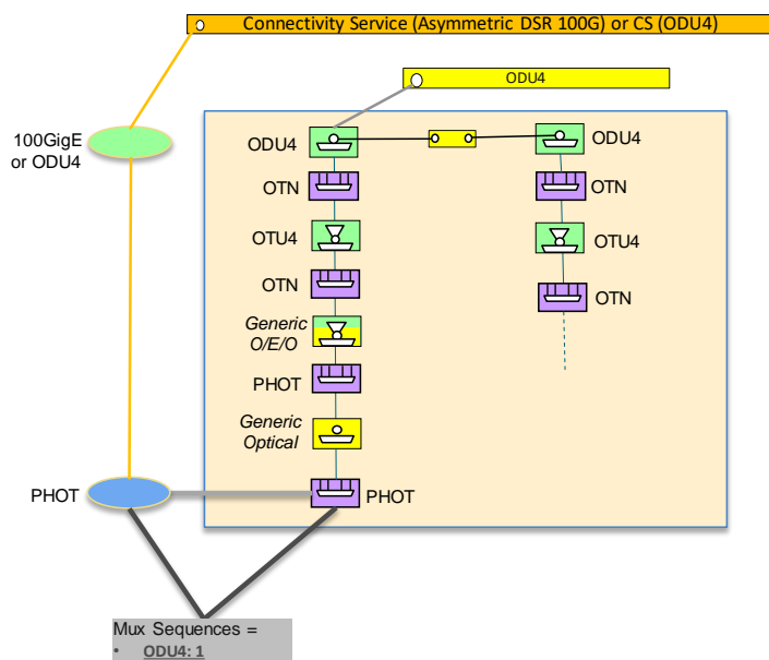
Figure 5-55 OTN ENNI, directly mapped client protocols, explicit model of functions
