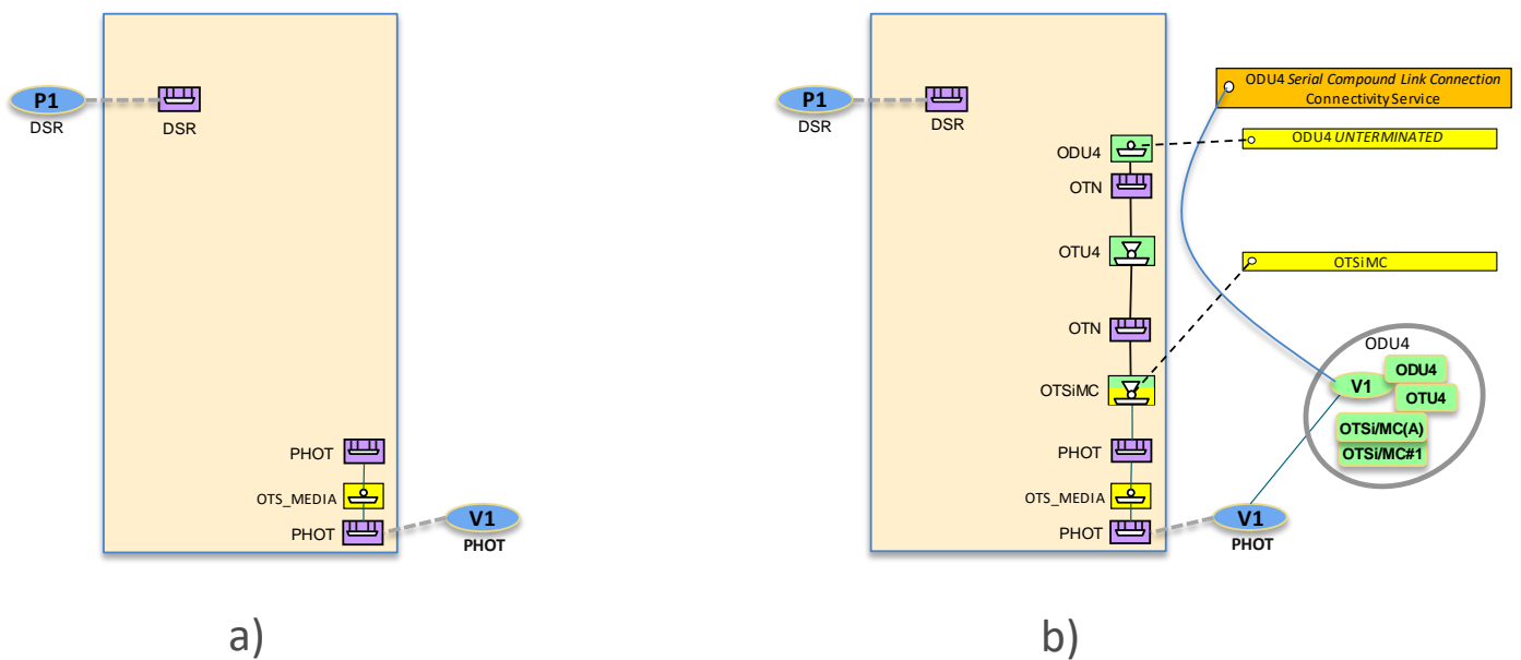
Figure 6-54 a) No server connections, b) Server ODU SCLC Connectivity Service
