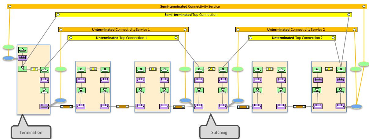
Figure 5-5 Unterminated Connection, semi-terminated CS and Connection
