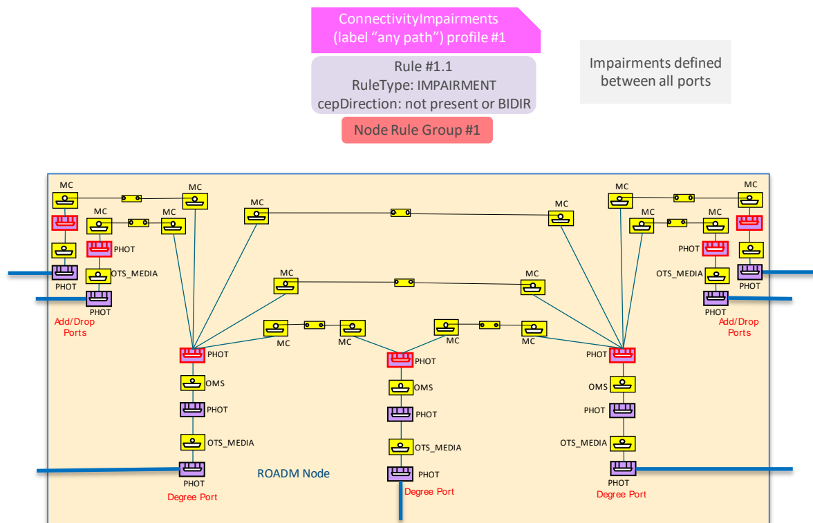
Figure 6-89 Connectivity Impairments are homogeneous for all potential connectivities
