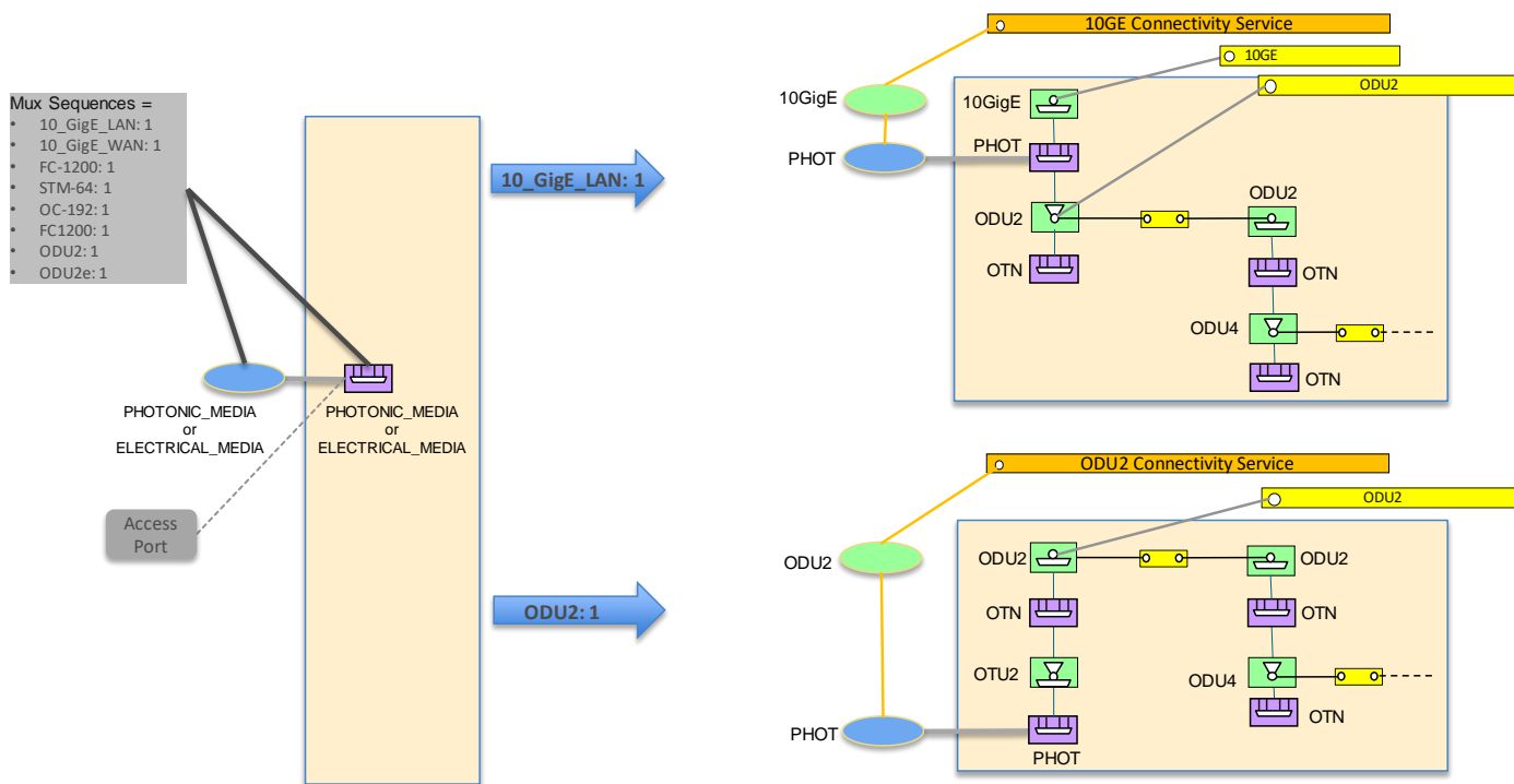
Figure 5-58 DSR/OTN NI, multi-technology interface, with OTU CEP in the OTN case
