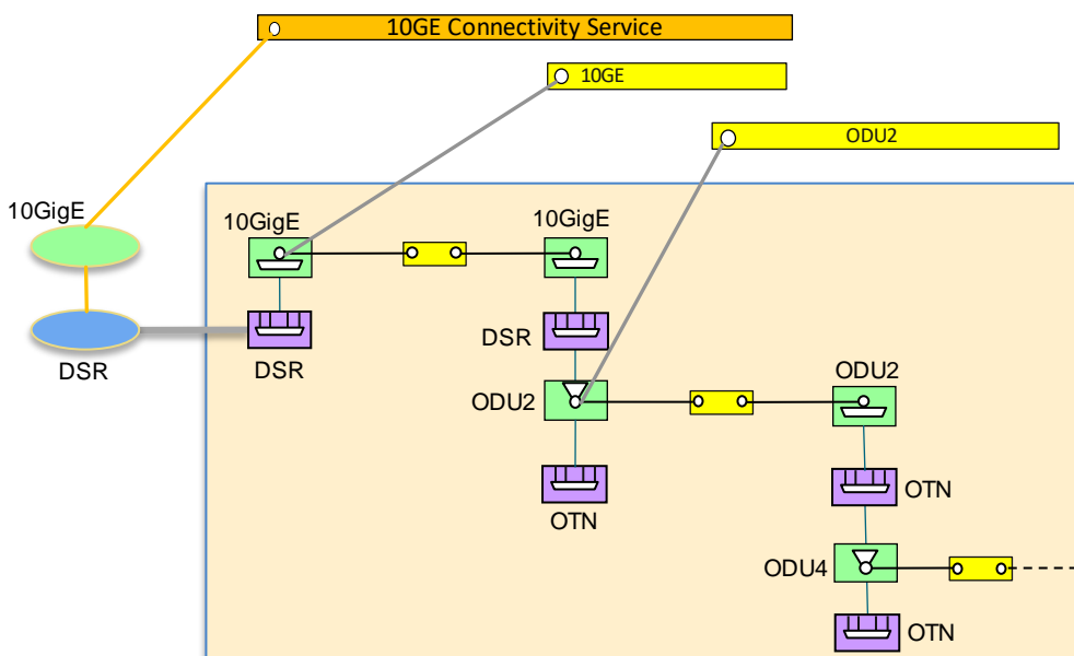
Figure 5-35 Option: Explicit DSR cross-connection
