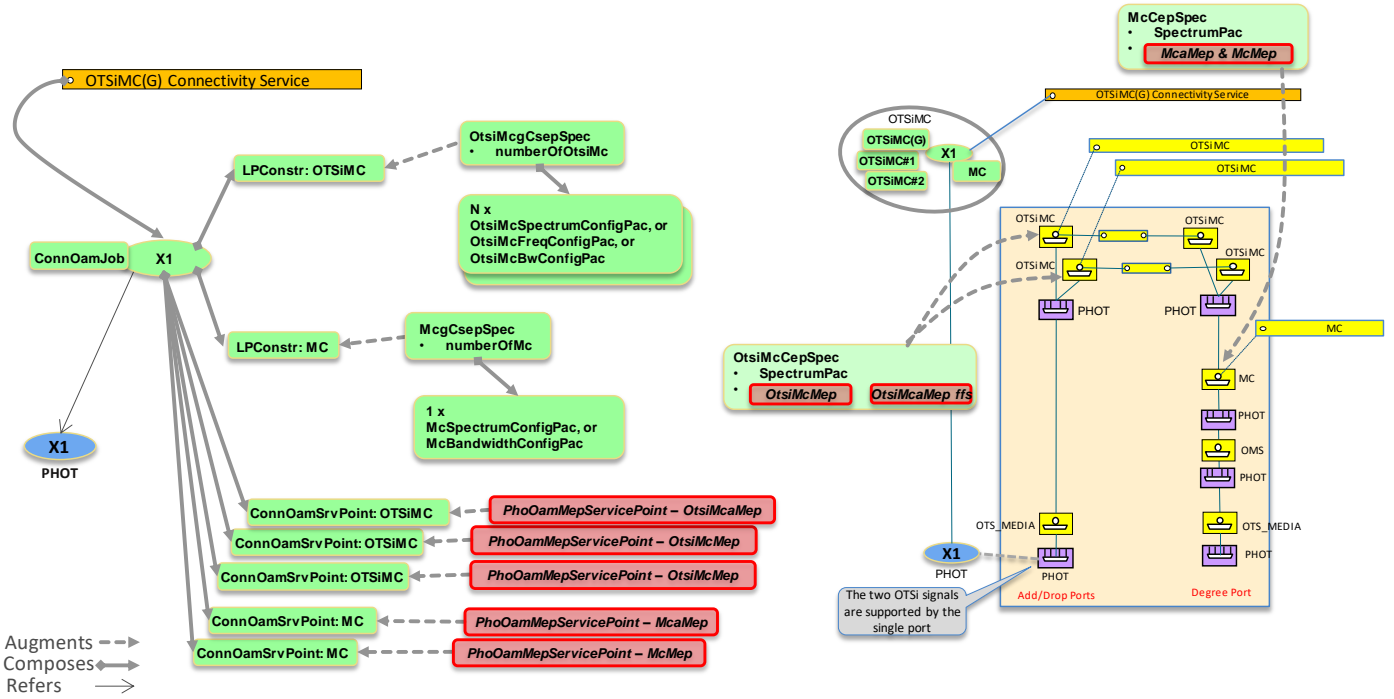
Figure 6-49 OTSiMC(G) CS on MC at Degree side, MC Connection automatically created or reused
