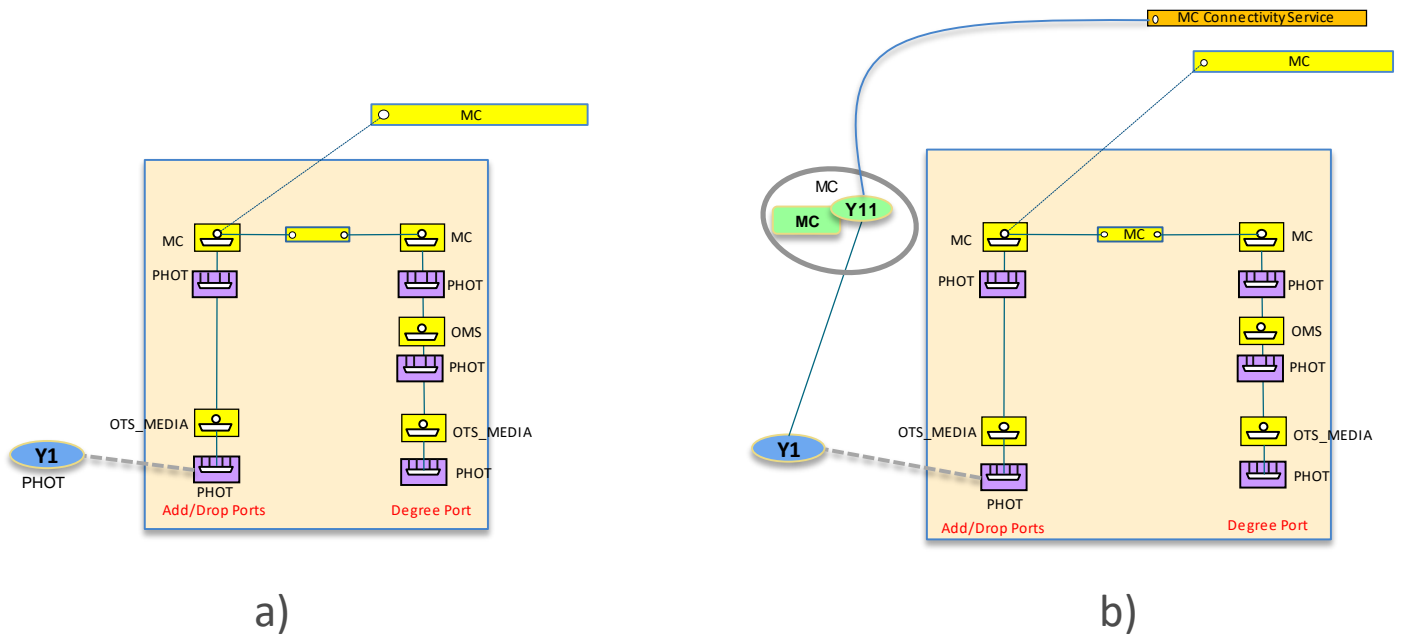
Figure 6-63 No “server” connections (auto creation of MC Conn/CS or no MC layer supported)
