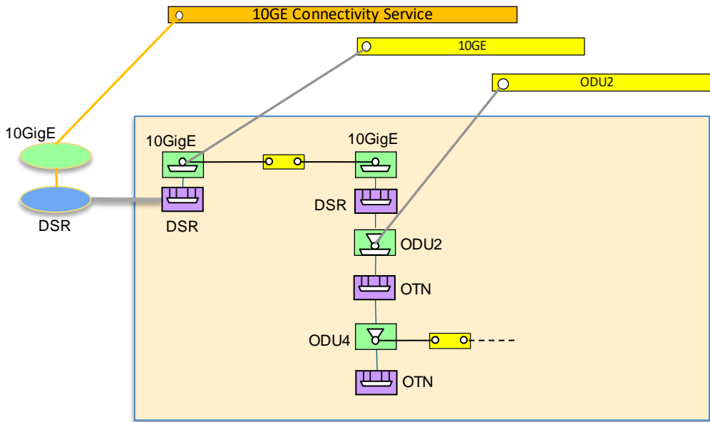
Figure 5-36 Option: Explicit DSR cross-connection, no ODU-LO cross-connection
