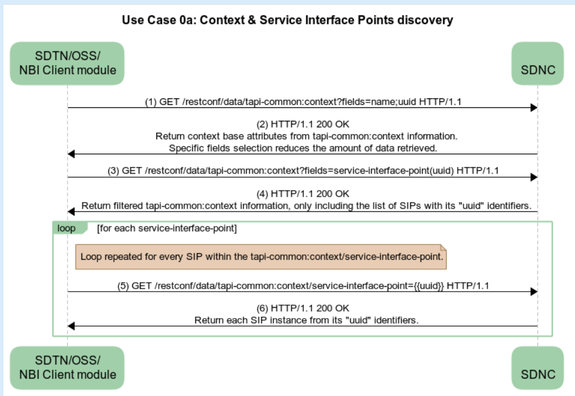
Figure 6-1 UC-0a: Context and Service Interface Point - Workflow.
