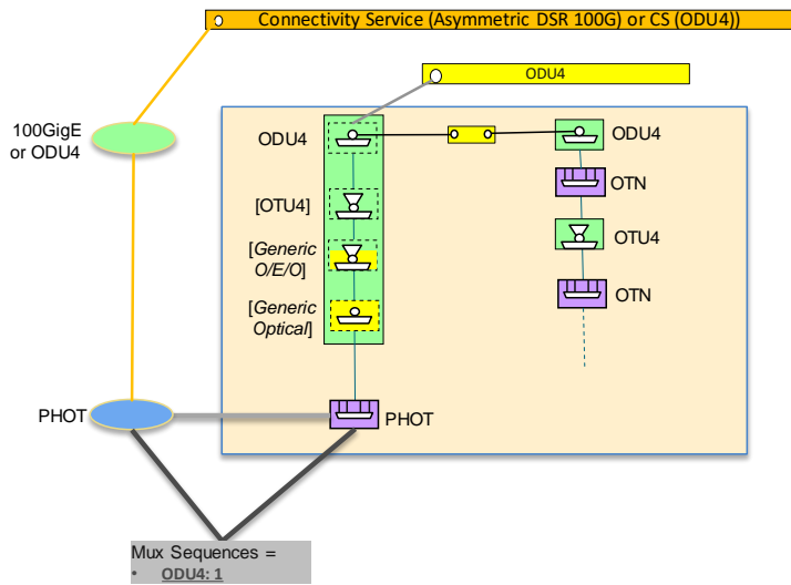
Figure 5-46 OTN ENNI, directly mapped client protocols, with additional embedded functions
