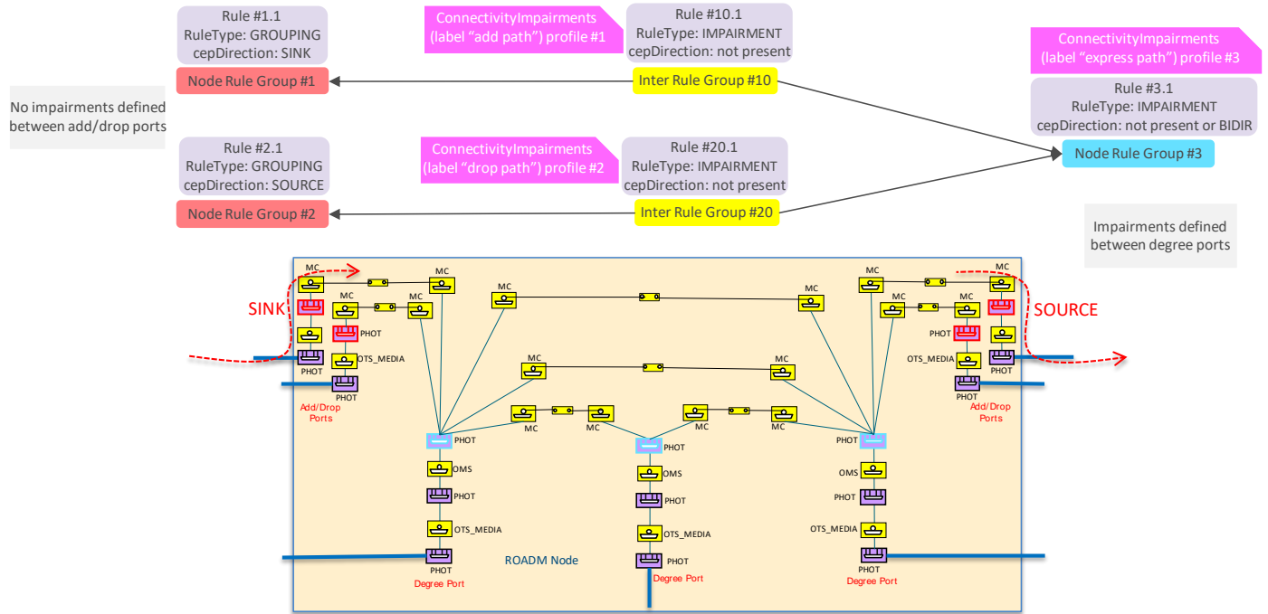
Figure 6-90 Conn. Impairments per add , drop and express conns, homogeneous between add / drop and express
