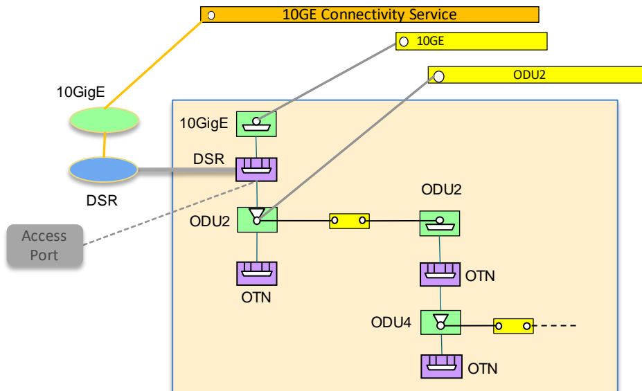
Figure 5-37 Option: No DSR cross-connection, with ODU-LO cross-connection
