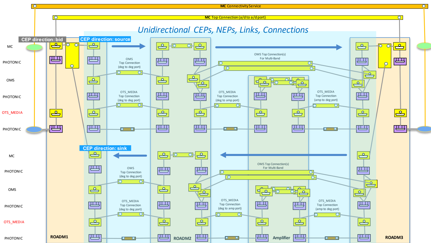
Figure 6-61 Mixed Scenario - UNI bidirectional and OMS unidirectional.
