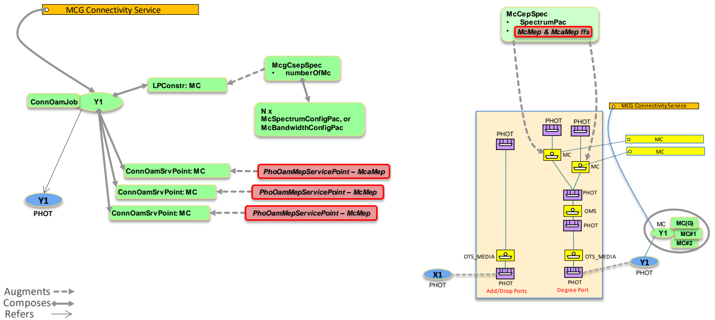
Figure 6-48 MCG Connectivity Service at Degree side
