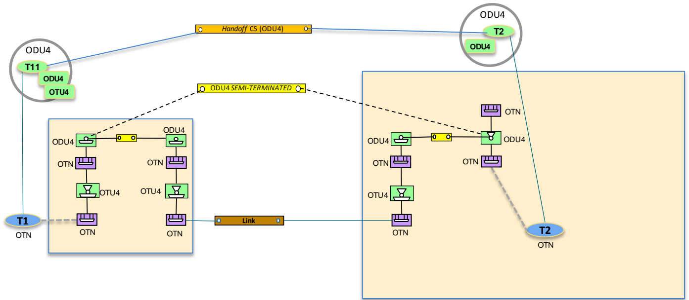
Figure 6-69 Server ODU Handoff Connectivity Service, variation
