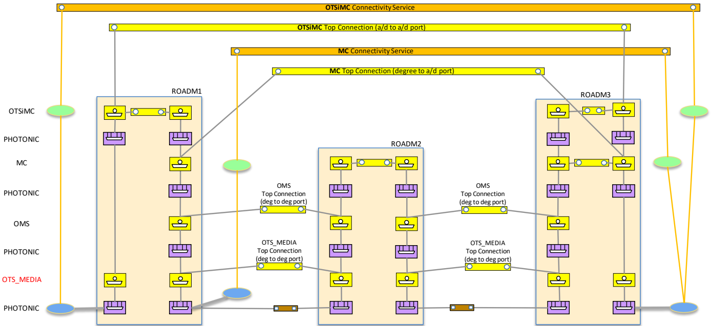
Figure 5-13 Scenario 1 : Optical Line System Controller, SIPs at both degree and a/d ports
