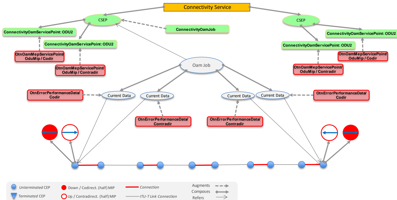
Figure 6-98 OAM provisioning, OTN NNI to NNI (unterminated)
