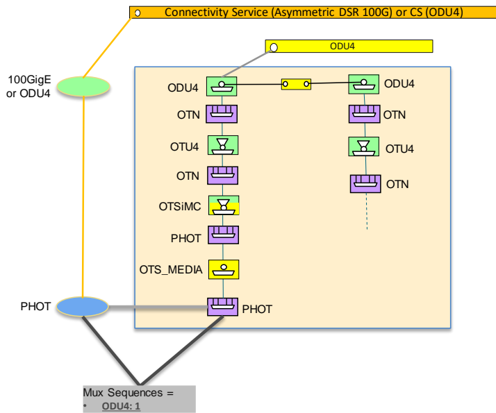
Figure 5-56 OTN ENNI, directly mapped client protocols, explicit model of defined functions
