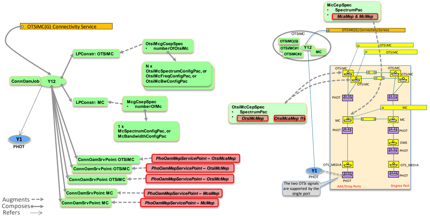
Figure 6-44 OTSiMCG CS on MC at Add/Drop side, MC Connection automatically created or reused
