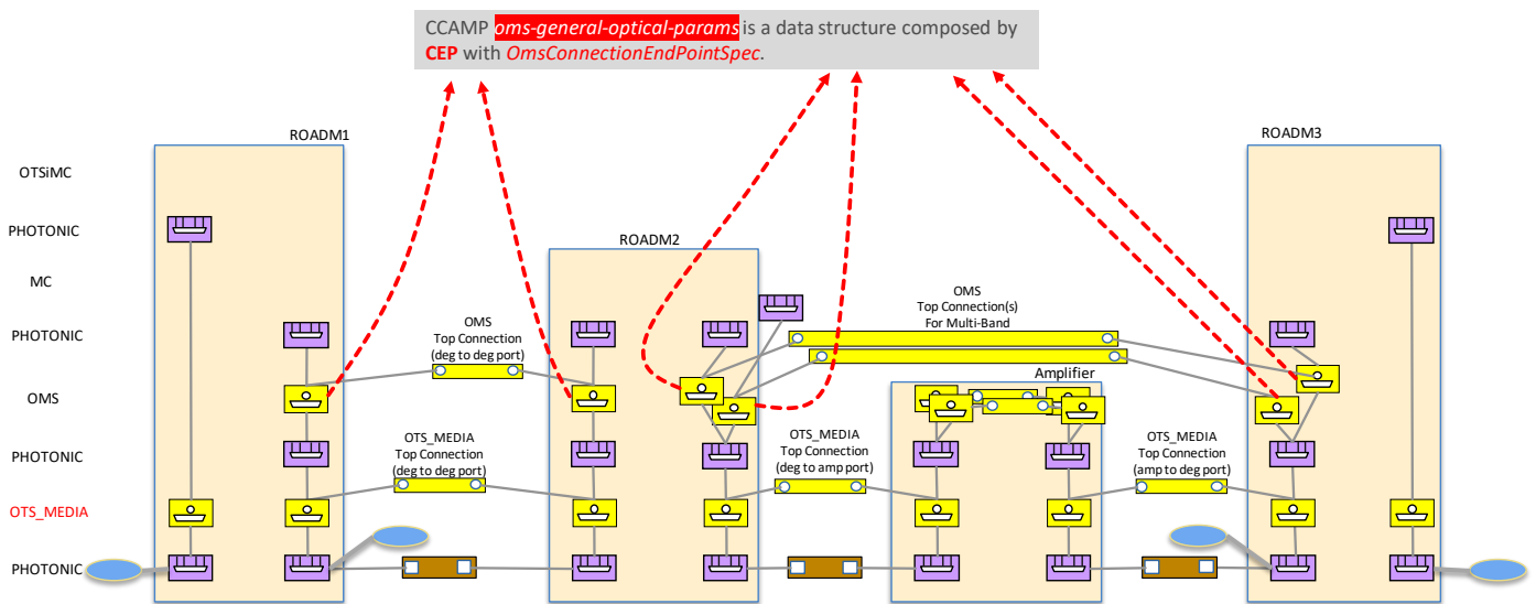
Figure 6-84 OMS Impairments
