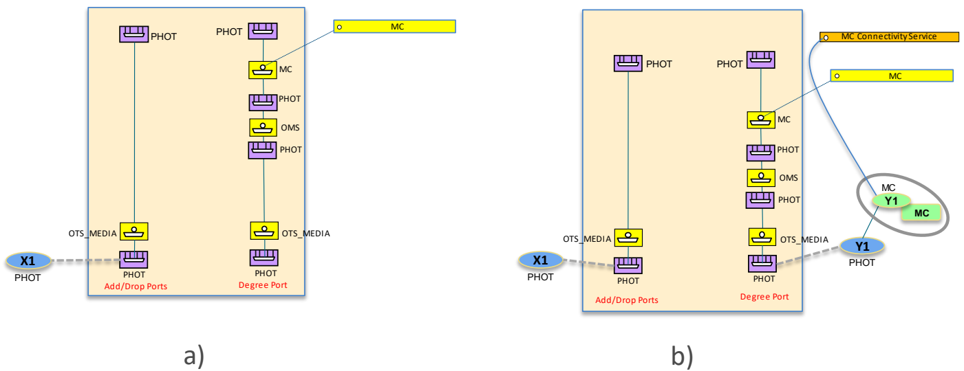
Figure 6-65 a) “Server” MC Connection at degree side, b) “Server” MC Connectivity Service at degree side
