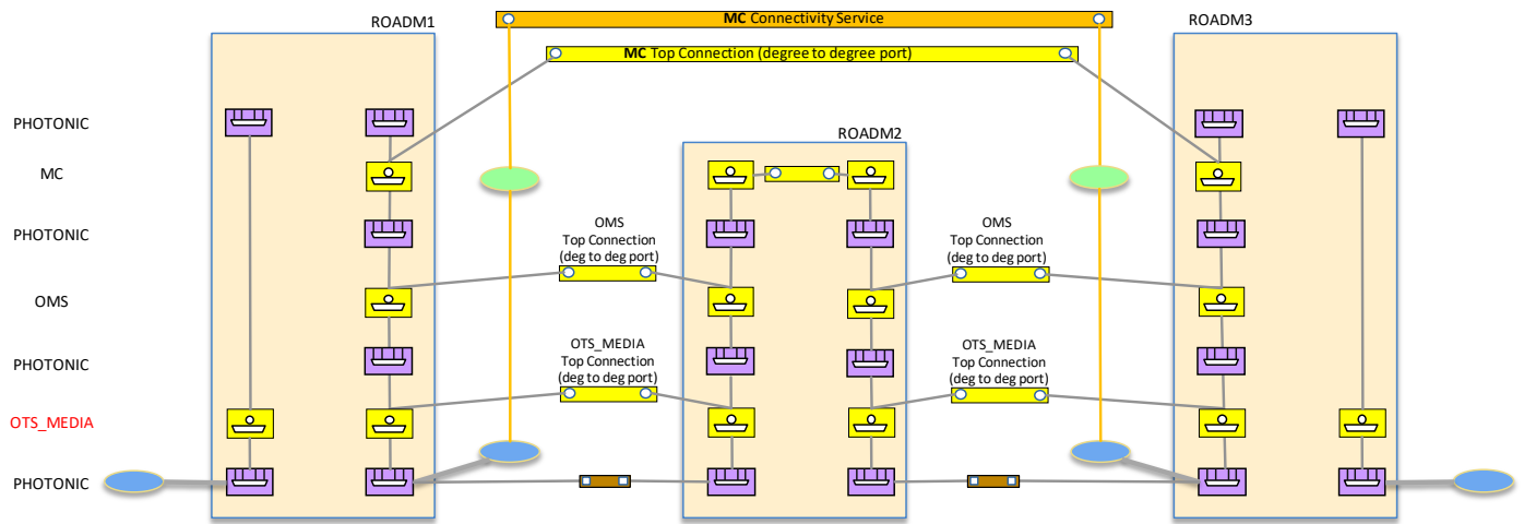
Figure 5-11 Scenario 1 : Optical Line System Controller, MC CS
