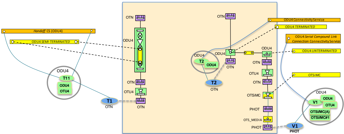
Figure 6-72 Server ODU Handoff Connectivity Service
