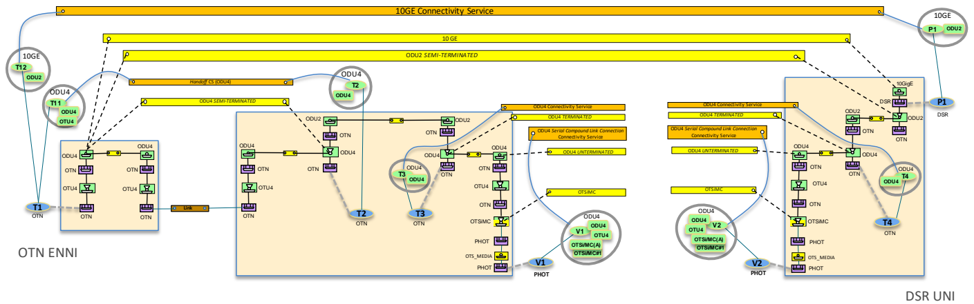
Figure 6-17 Asymmetric Scenario 1: Handoff at ODU4 Layer, ODU2 layer switching on Edge Node, variation
