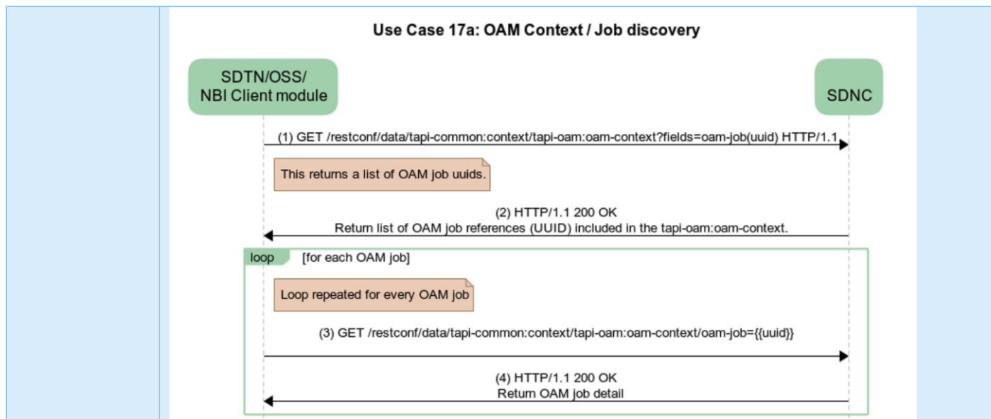
Figure 6-105 UC-17a: OAM Context discovery
