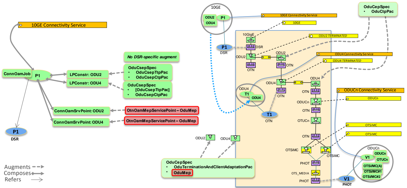
Figure 6-36 DSR/ODUj CS on ODUk CS on ODUCn CS - Auto creation of ODUk CS
