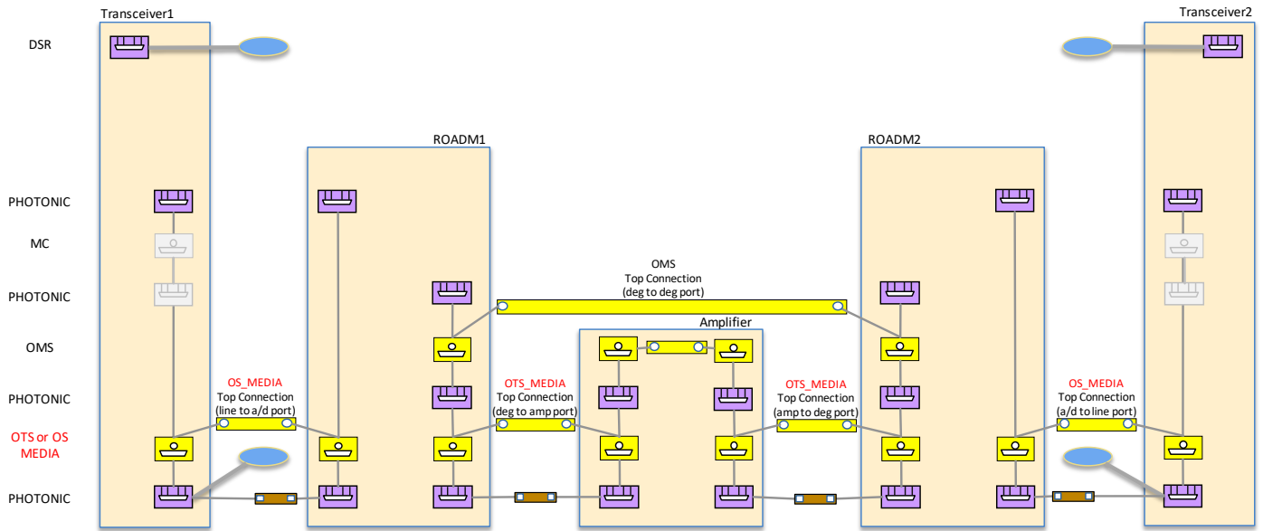
Figure 5-18 Scenario 2 : Integrated Management, time zero, OS_MEDIA
