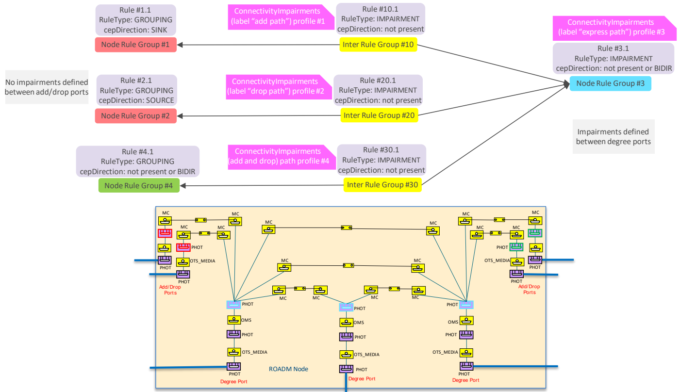
Figure 6-91 Conn. Impairments per add , drop and express conns, not homogeneous between add / drop and express
