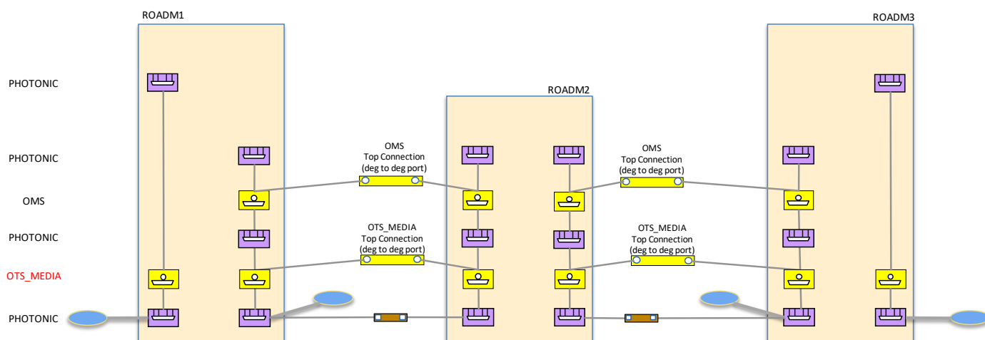
Figure 5-10 Scenario 1 : Optical Line System Controller, time zero, SIPs also on degree ports
