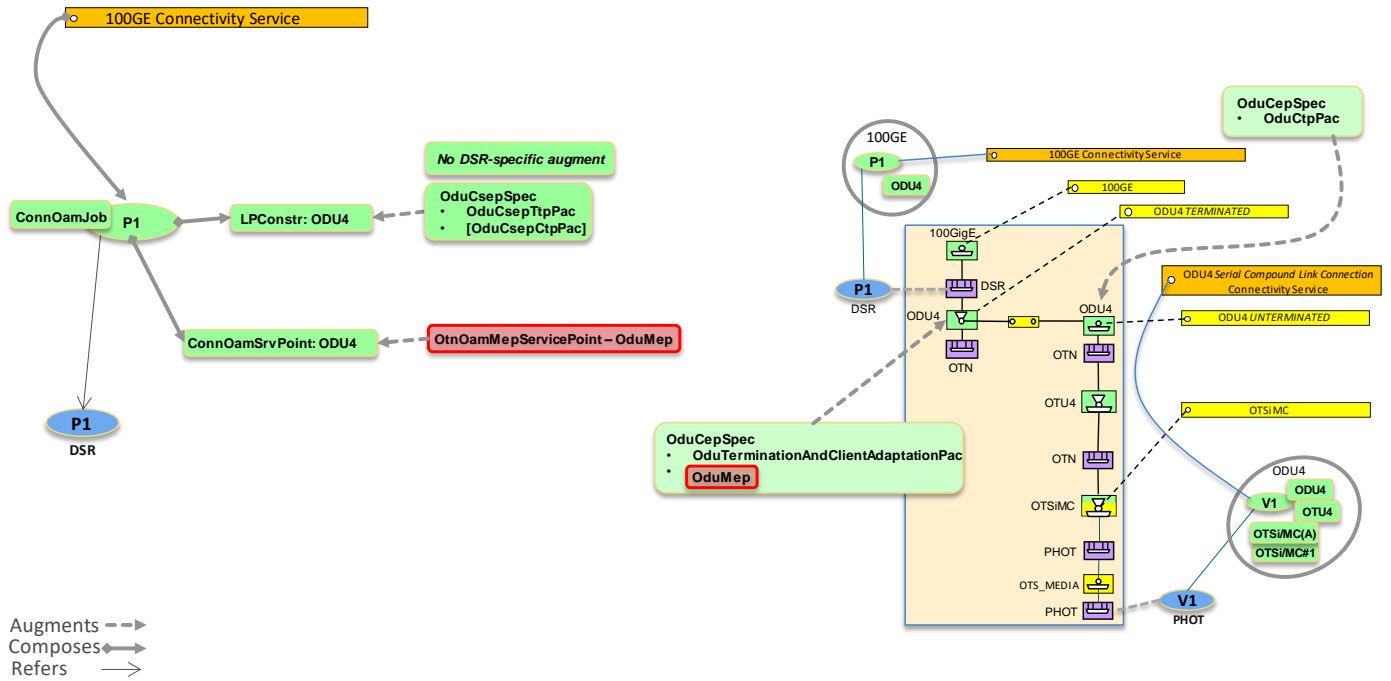
Figure 6-9 DSR/ODUk Connectivity Service on ODUk SCLC CS
