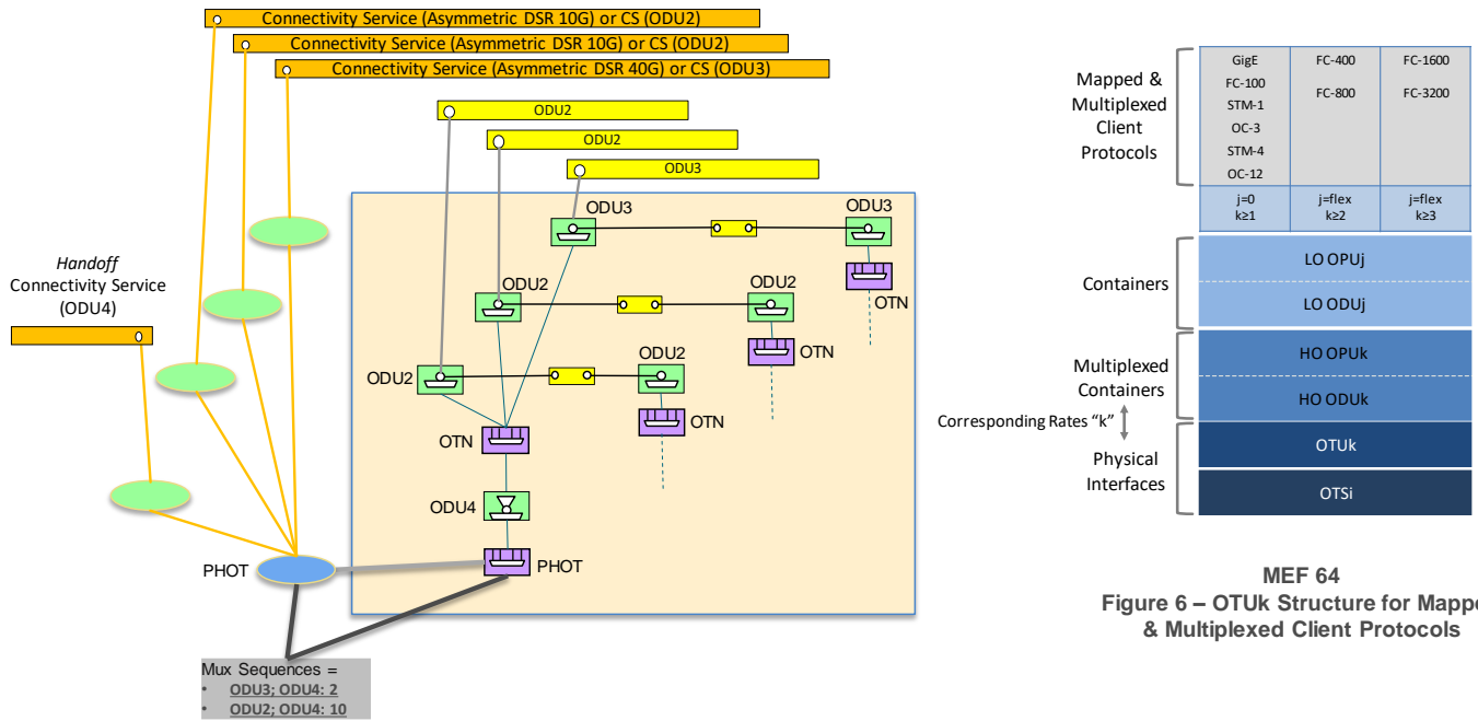
Figure 5-48 OTN ENNI, mapped & multiplexed client protocols
