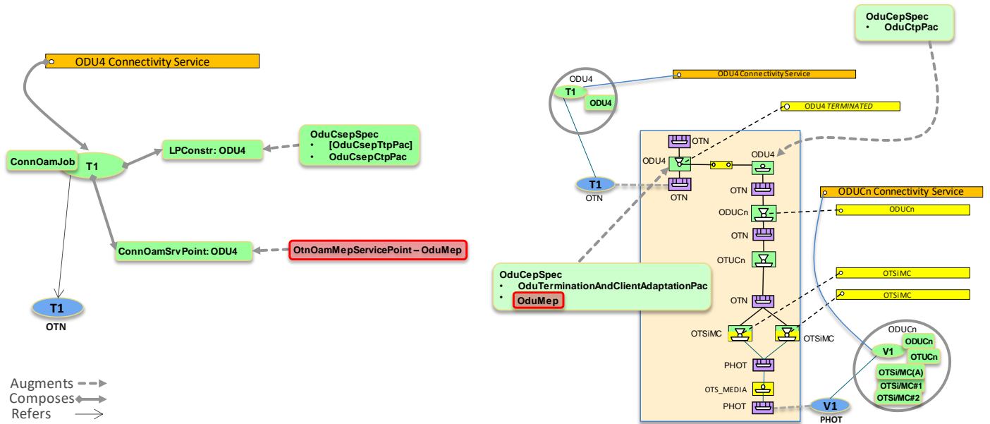
Figure 6-37 Infrastructure or Handoff ODUk CS on ODUCn CS
