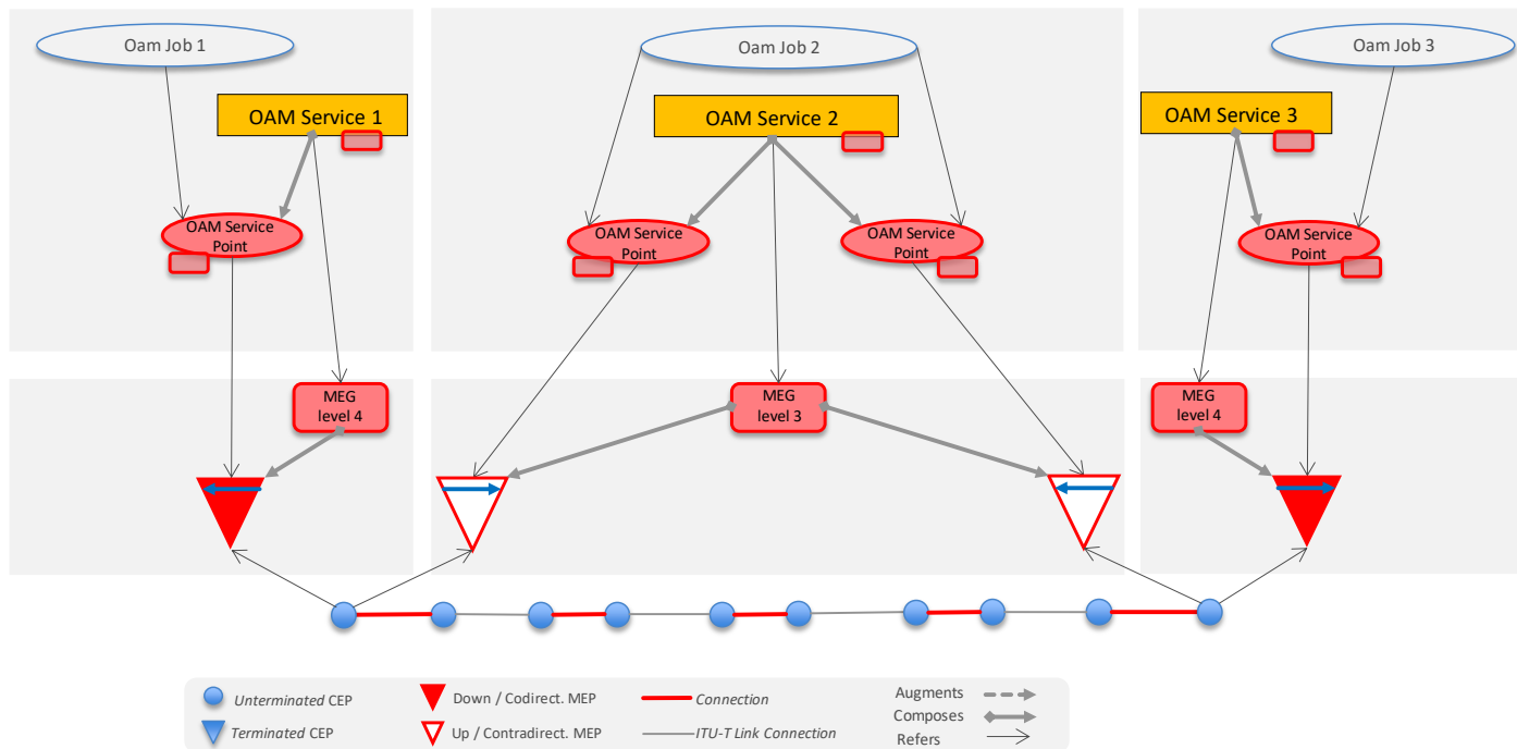
Figure 6-101 OAM Provisioning, Client Controller creates the OAM Jobs
