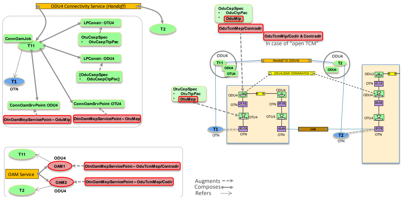
Figure 6-21 Asymmetric scenario 1: ODUk Handoff CS (OTN ENNI) – Part 1
