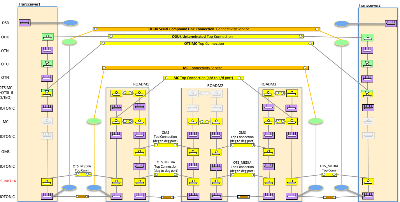
Figure 5-21 Scenario 2 : Integrated Management, MC and OTSICM+ODU CSs
