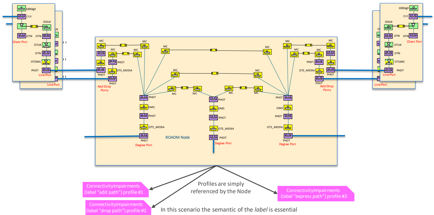
Figure 6-88 Connectivity Impairments – No Node Rule Group
