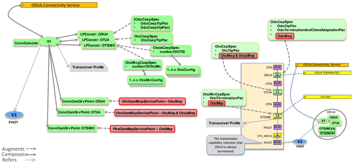
Figure 6-39 ODUk Trail Connectivity Service
