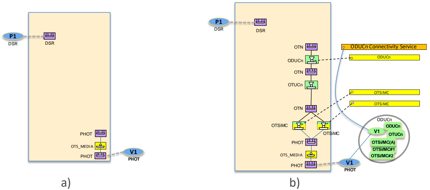
Figure 6-57 a) No server connections, b) Server ODUcN Connectivity Service
