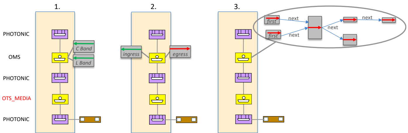
Figure 6-87 More Amplification functions per CEP instance
