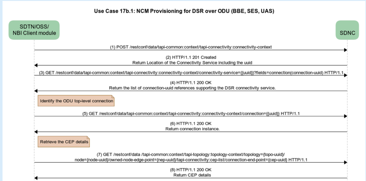
Figure 6-107 UC-17b.1: NCM DSR over ODU with BBE, SES, UAS
