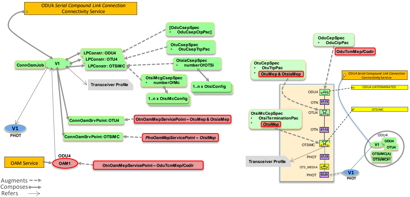
Figure 6-8 ODUk Serial Compound Link Connection Connectivity Service
