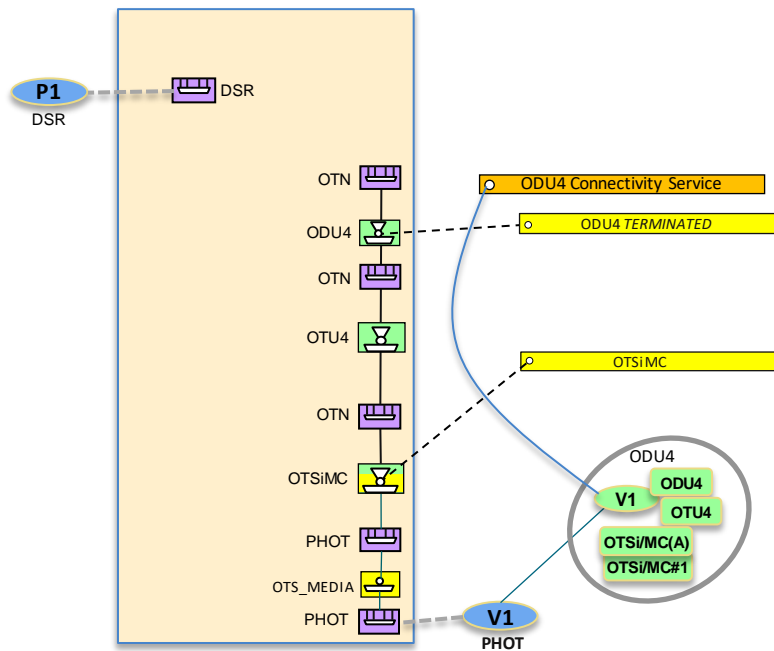
Figure 6-55 a) Server ODU SCLC CS and HO ODU connection, b) Server ODU SCLC CS and HO ODU CS
