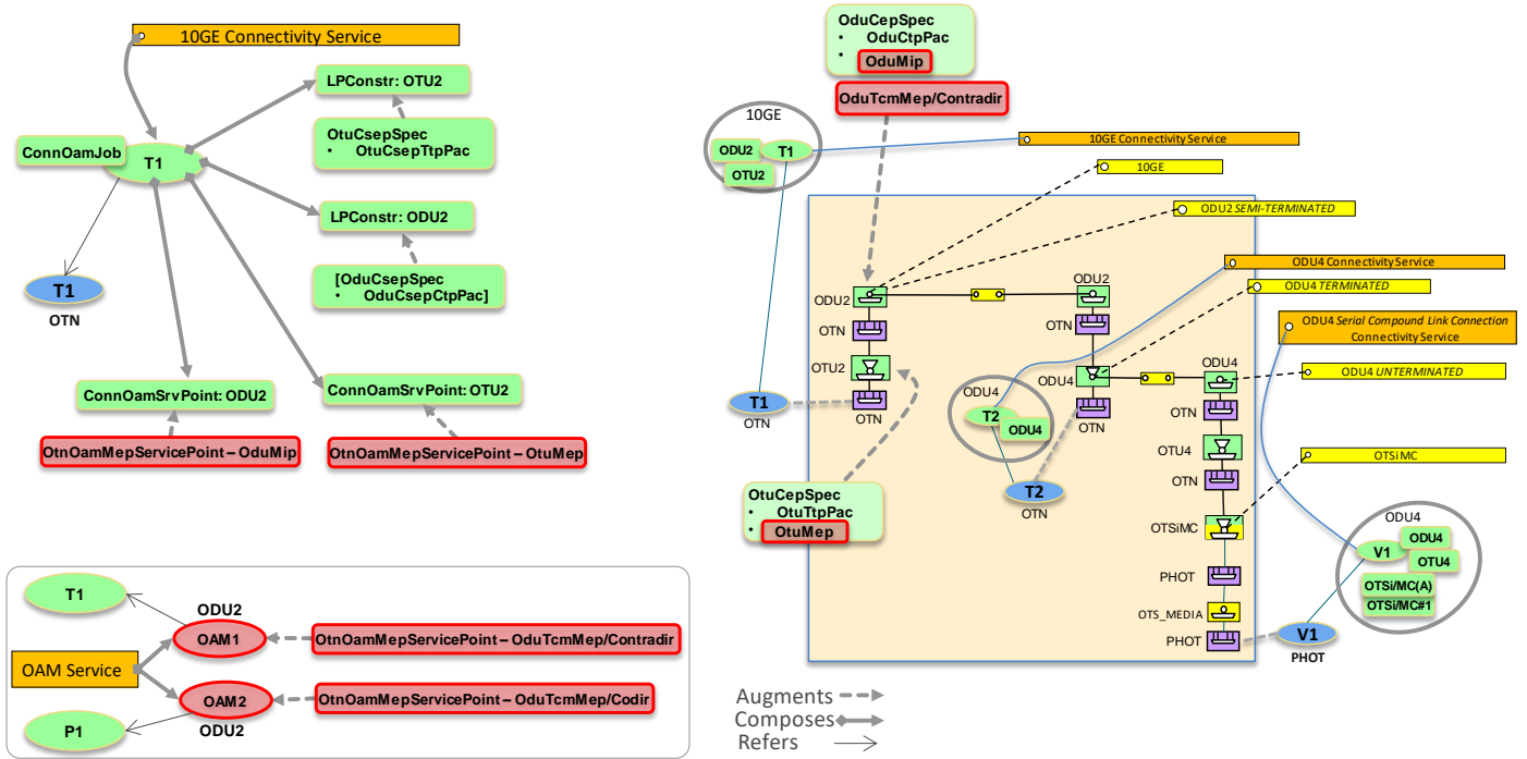
Figure 6-30 Asymmetric scenario 3: DSR/ODUj CS (OTN ENNI)
