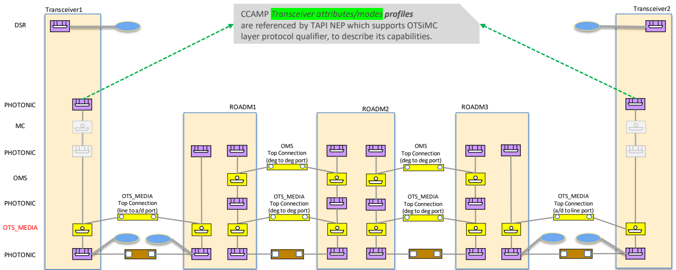
Figure 6-82 Transceiver Profile, capability
