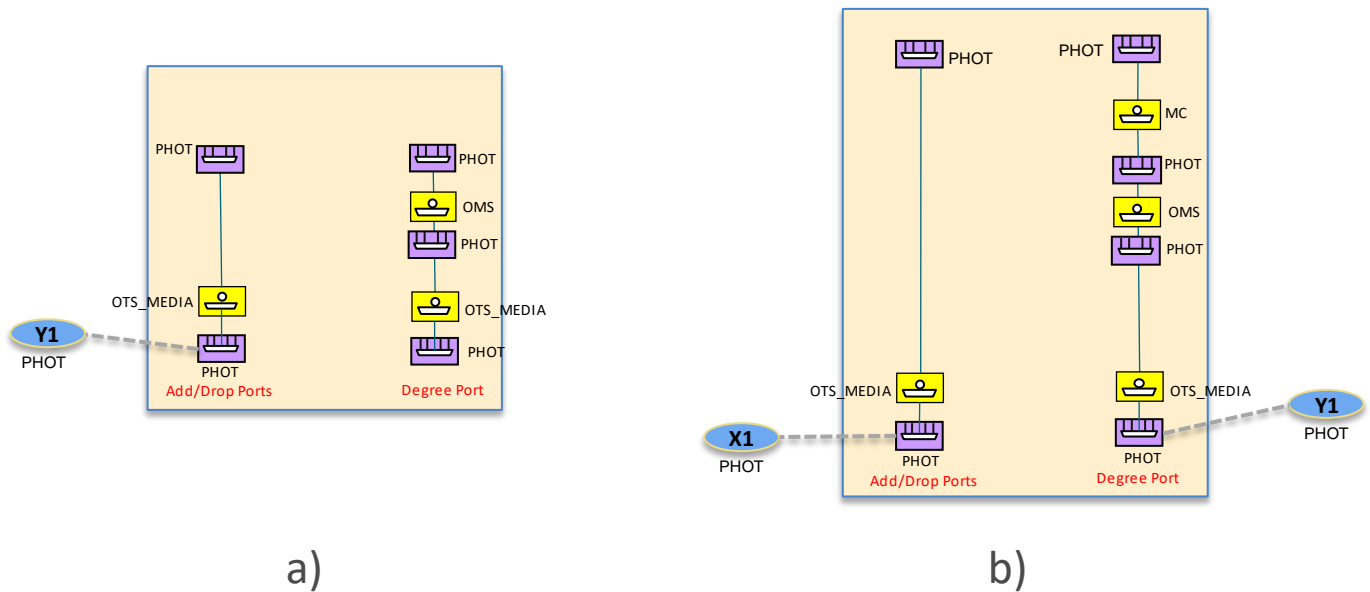
Figure 6-60 a) MC CS at Add/Drop side, b) MC CS at Degree side (Y1 SIP)
