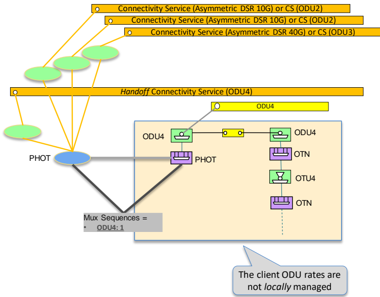
Figure 5-52 OTN ENNI, not locally mapped & multiplexed client protocols
