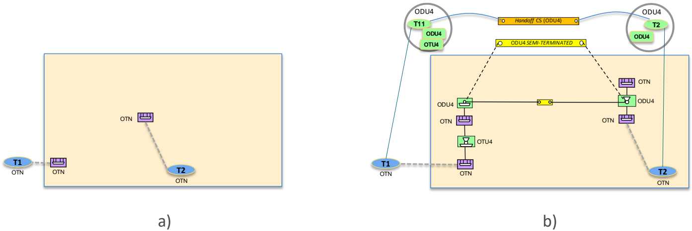
Figure 6-70 a) No “server” connections, b) Server ODU Handoff Connectivity Service
