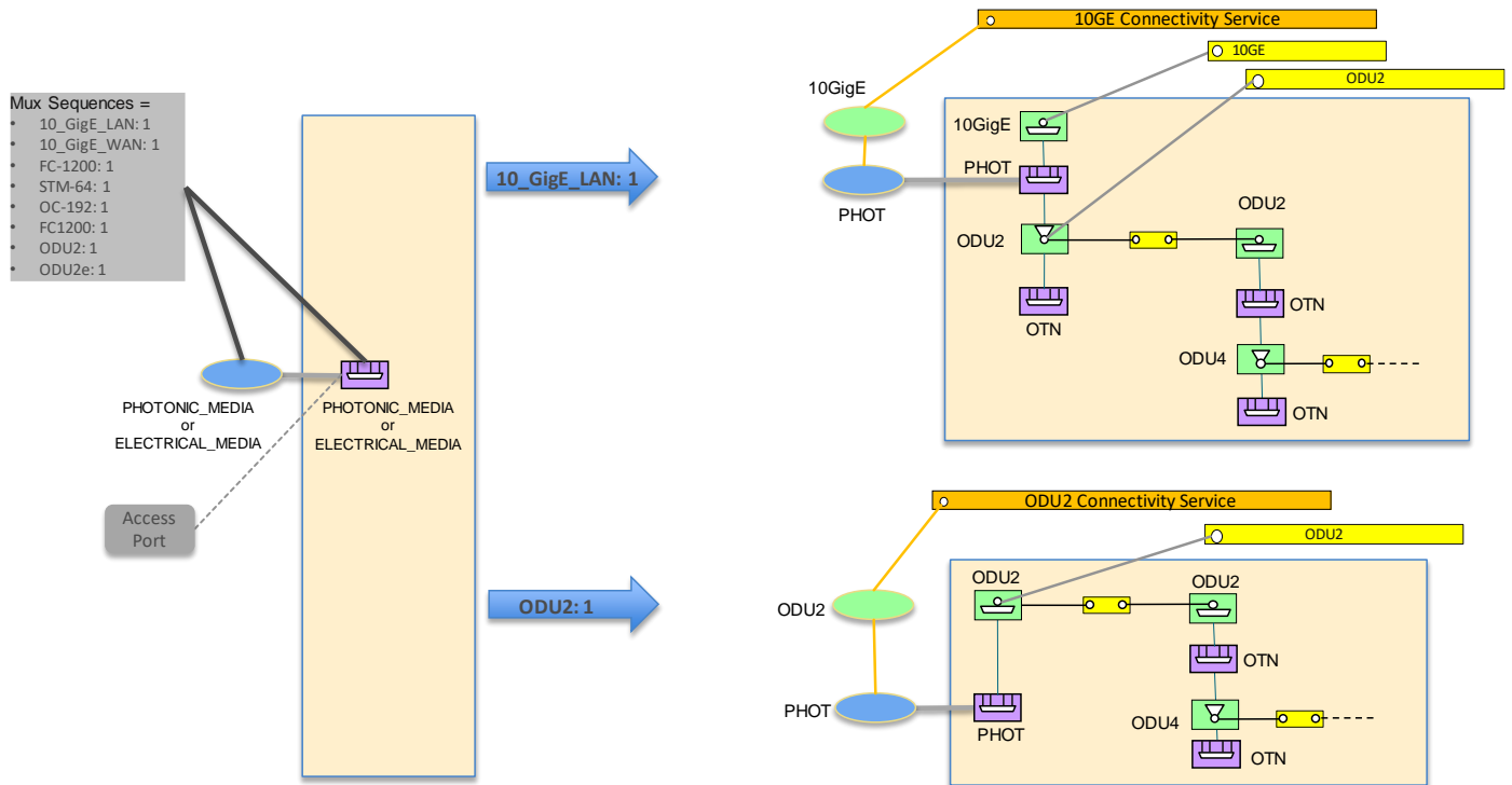
Figure 5-57 DSR/OTN NI, multi-technology interface
