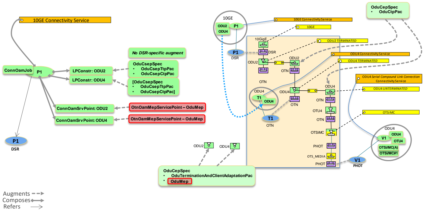
Figure 6-13 DSR/ODUj Connectivity Service on ODUk SCLC CS, auto creation of ODUk CS
