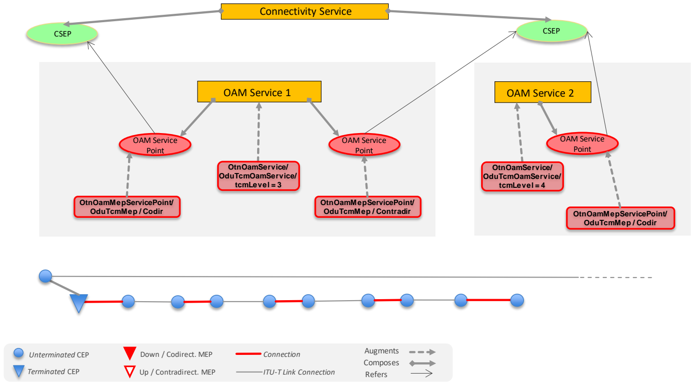
Figure 6-103 OAM provisioning, Client Controller creates the OAM Service and its End Points, DSR UNI to NNI
