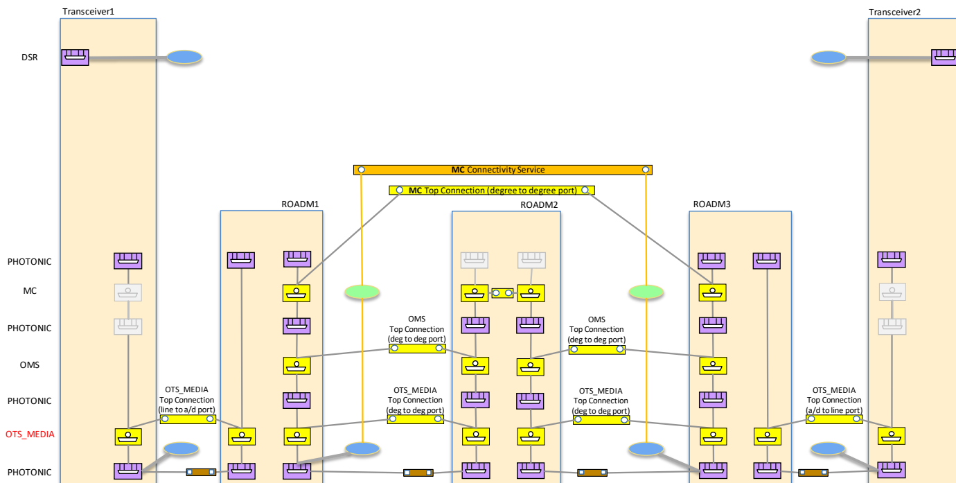
Figure 5-27 Scenario 2 : Integrated Management, MC CS
