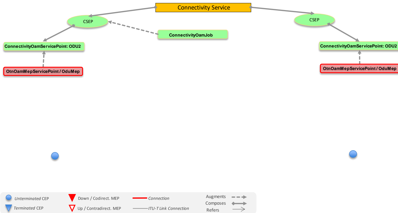
Figure 6-95 OAM provisioning, Client Controller creates the CS with the CSEPs including OAM configuration
