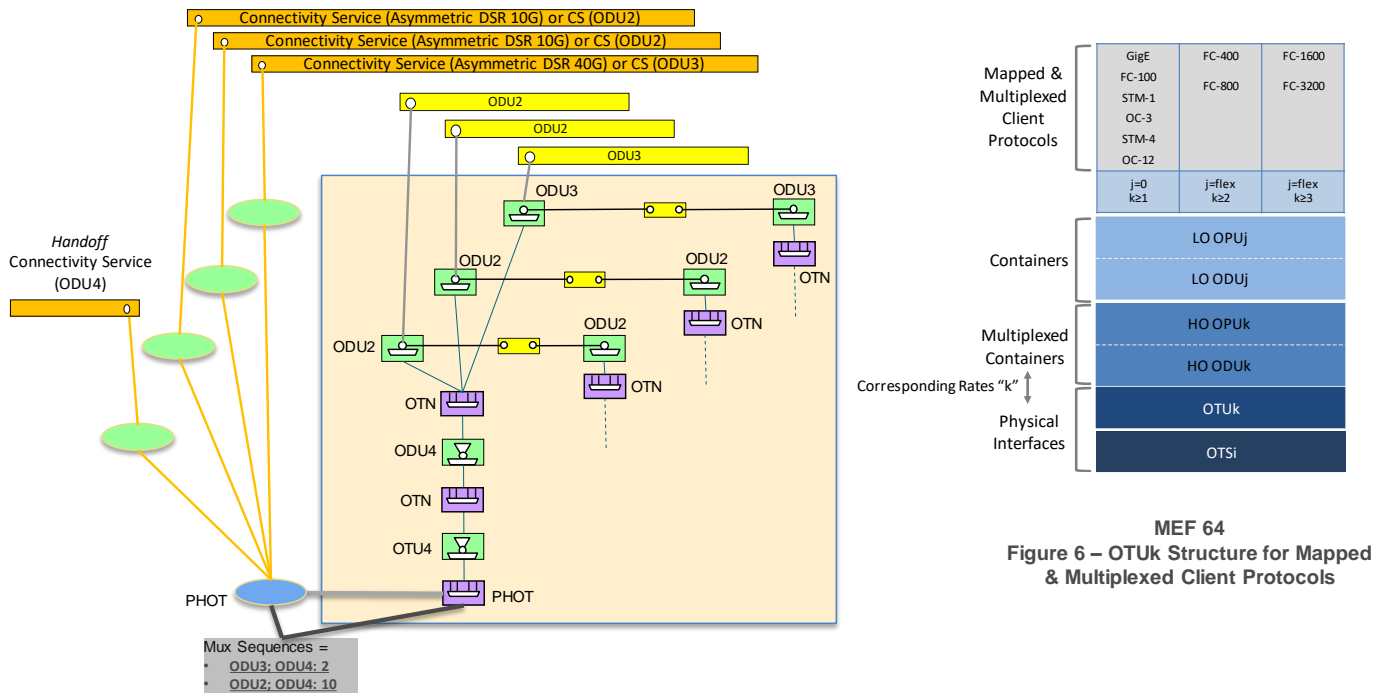
Figure 5-49 OTN ENNI, mapped & multiplexed client protocols, with OTU CEP
