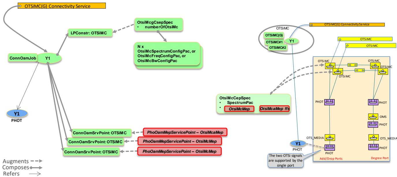
Figure 6-52 OTSiMC Connectivity Service without MC Layer
