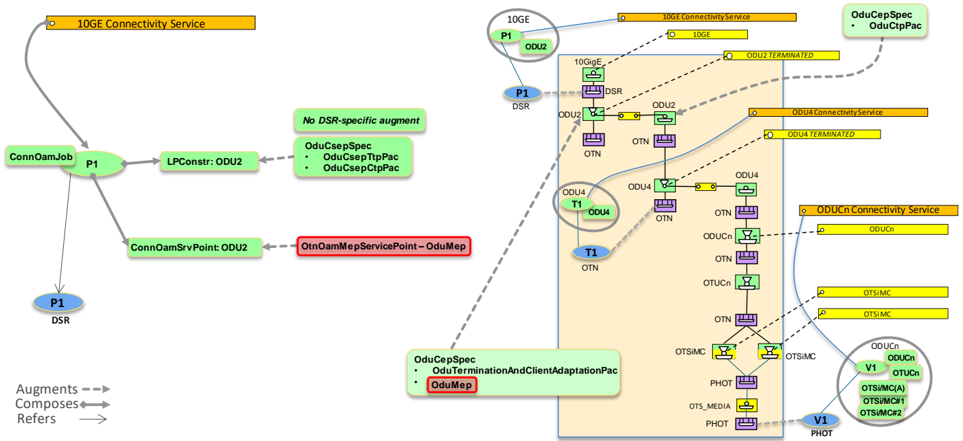
Figure 6-38 DSR/ODUj CS on ODUk CS on ODUCn CS
