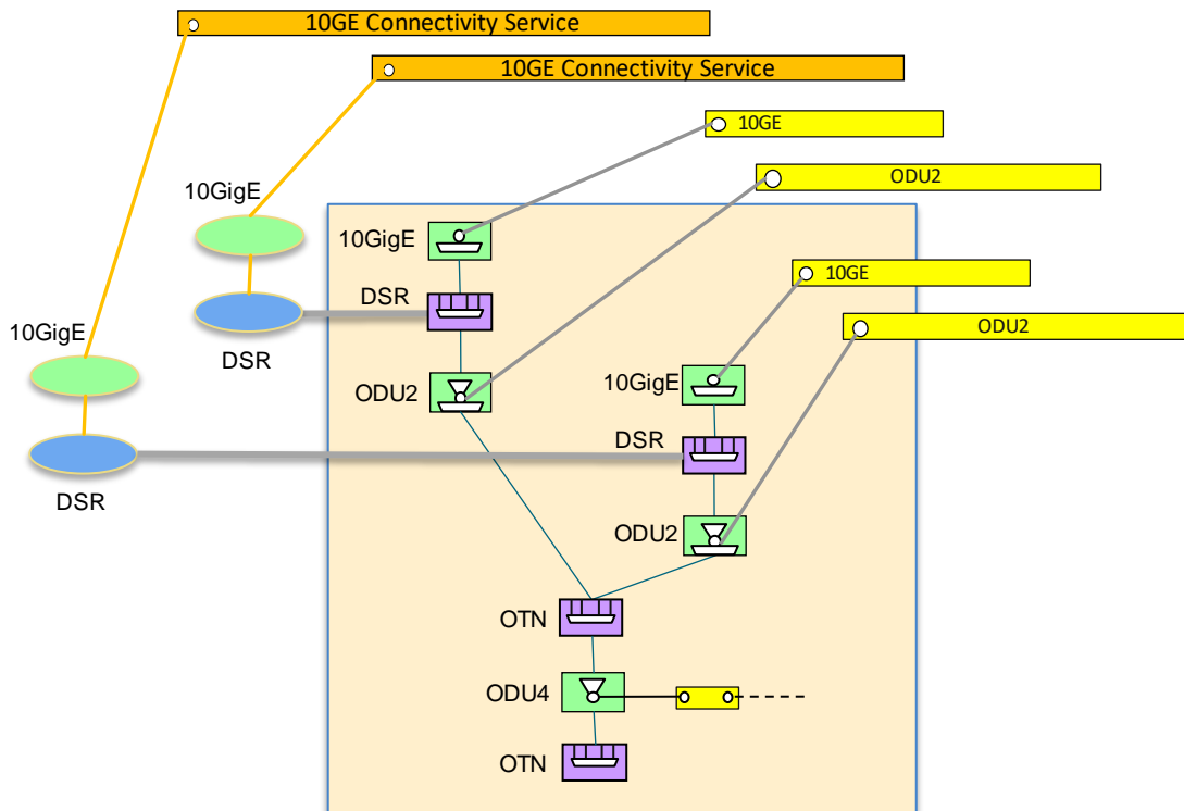
Figure 5-38 Option: No DSR/ODU-LO cross-connections
