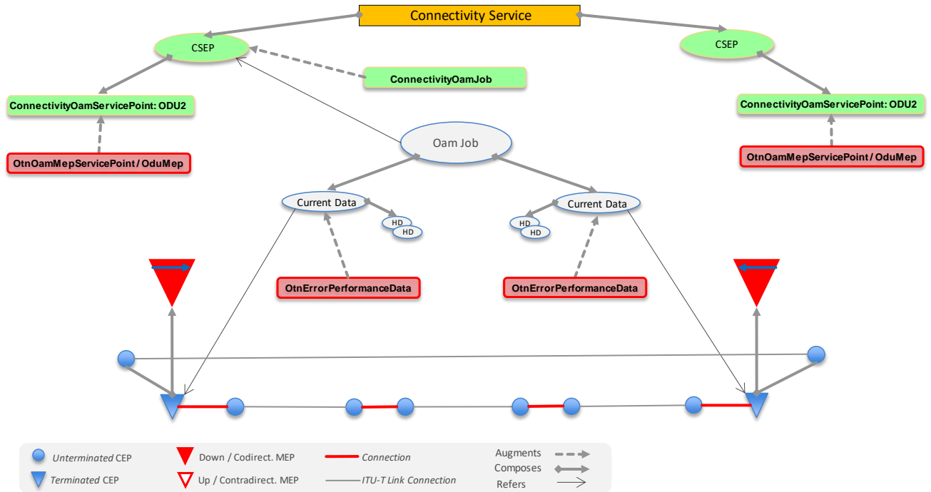
Figure 6-96 OAM provisioning, Server Controller creates OAM Job, Current and History Data instances
