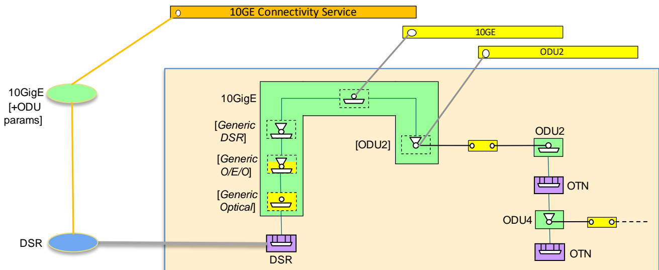
Figure 5-40 Option: Simplified DSR UNI with additional embedded functions
