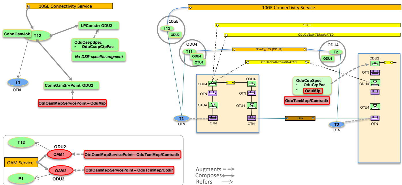
Figure 6-23 Asymmetric scenario 1: DSR/ODUj CS (OTN ENNI)
