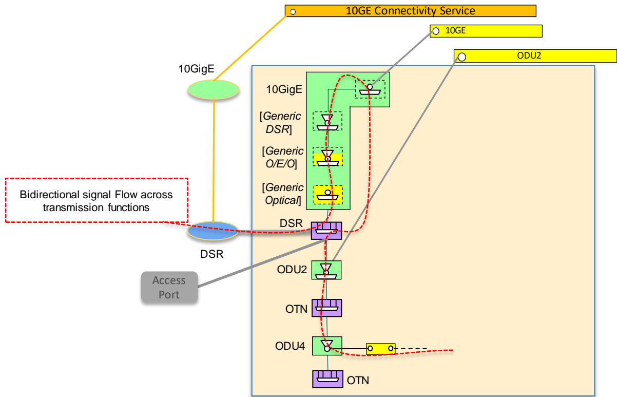
Figure 5-41 Option: DSR UNI with additional embedded functions with explicit DSR and ODU cross-connections (top), simplified without DSR cross-connection (middle), and simplified without cross-connections (bottom)
