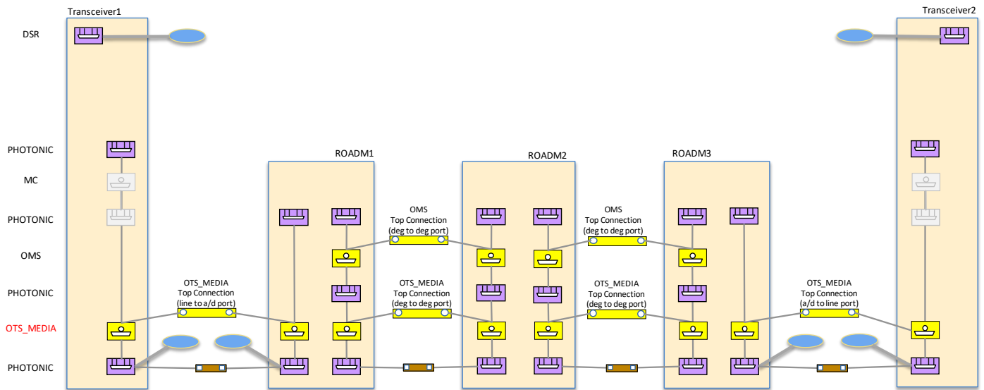
Figure 5-19 Scenario 2 : Integrated Management, time zero, SIPs at a/d ports
