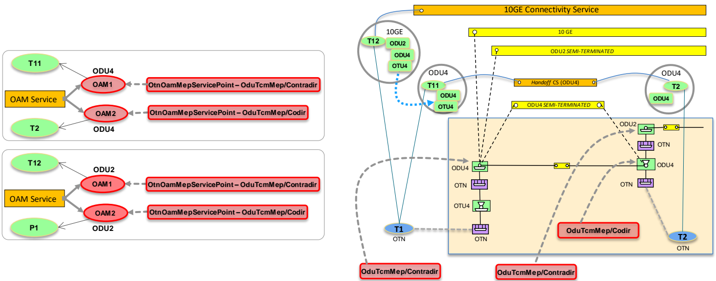
Figure 6-29 Asymmetric scenario 2: DSR/ODUj CS (OTN ENNI) - Auto creation of ODUk Handoff CS – Part 2
