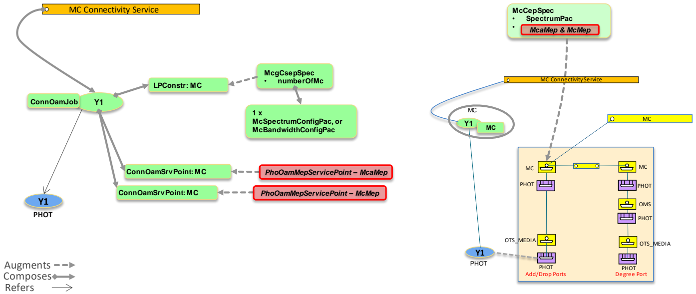
Figure 6-42 MC Connectivity Service at Add/Drop side
