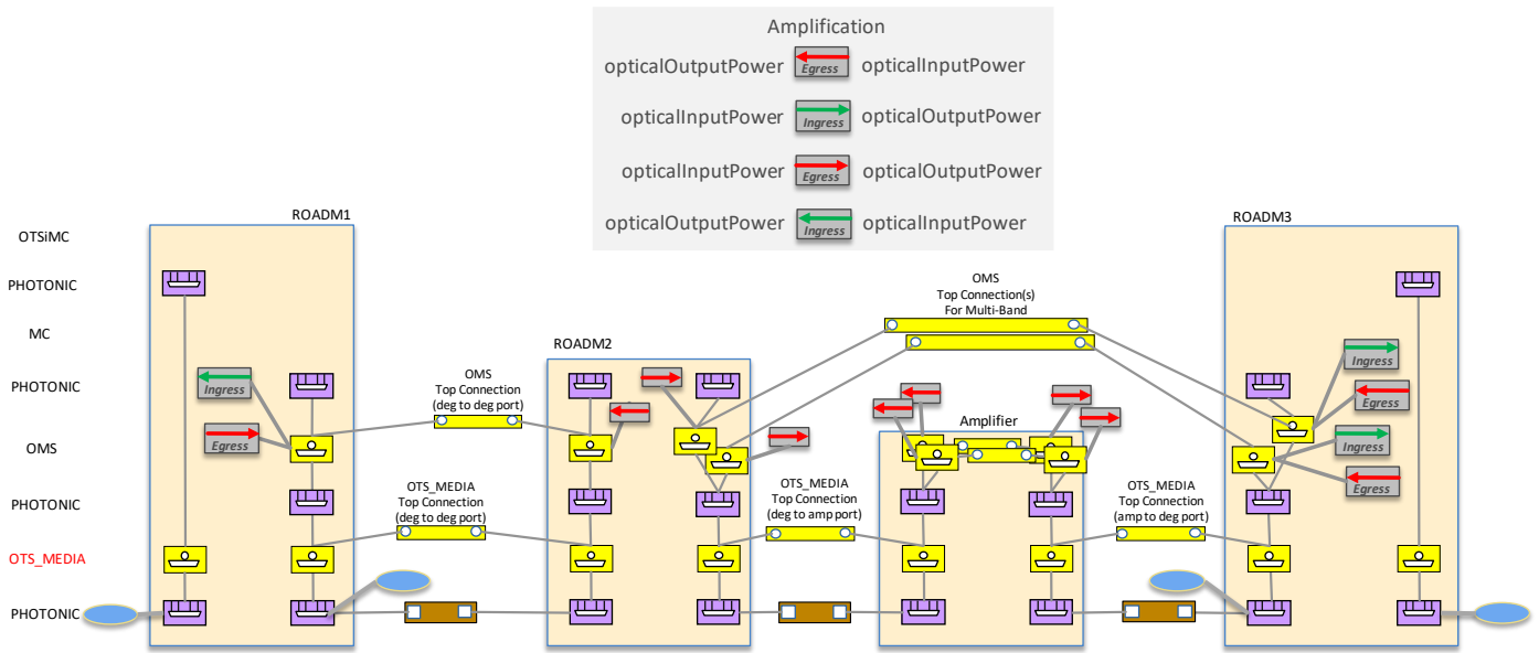
Figure 6-86 Amplification Impairments
