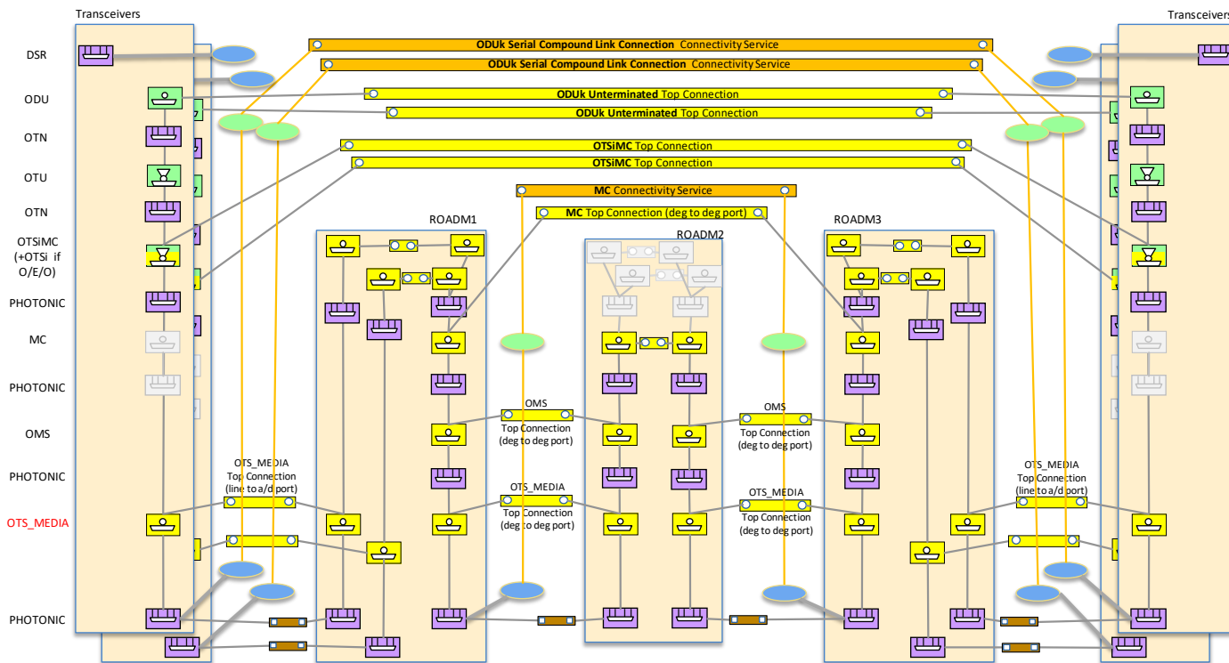
Figure 5-30 Scenario 2 : Integrated Management, MC and OTSiMC+ODU CSs, more OTSiMCs on MC
