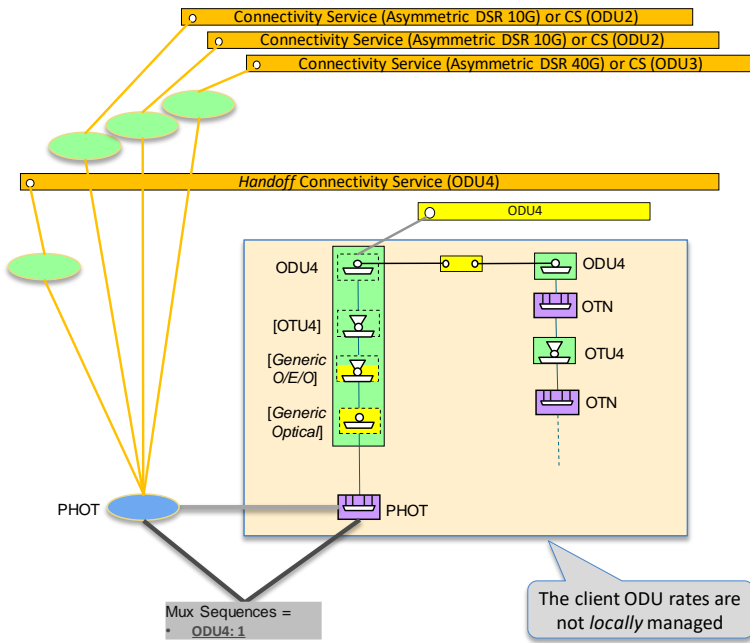
Figure 5-54 OTN ENNI, not locally mapped & multiplexed client protocols, with additional embedded functions
