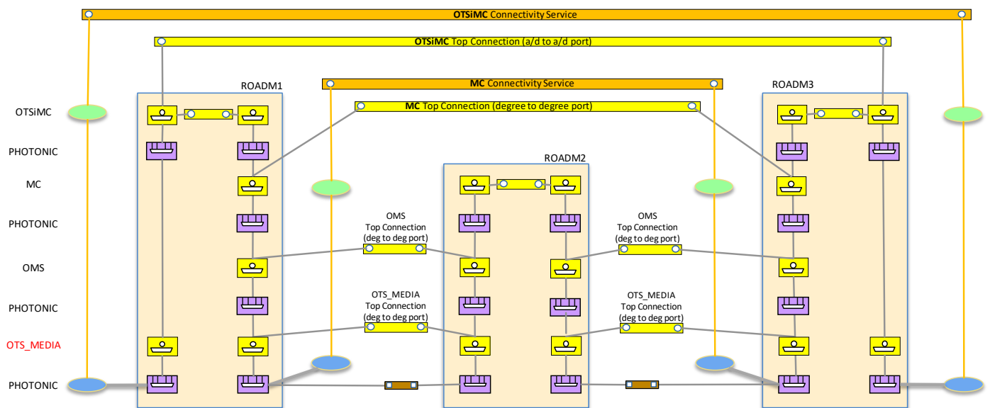
Figure 5-12 Scenario 1 : Optical Line System Controller, OTSiMC and MC CSs
