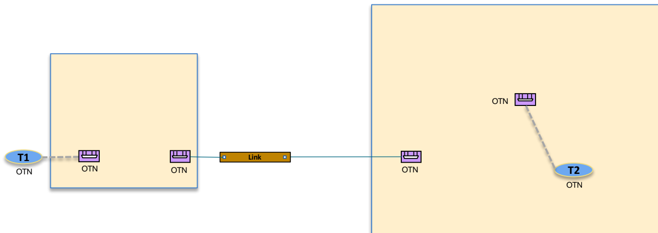
Figure 6-68 No "server" connections, variation
